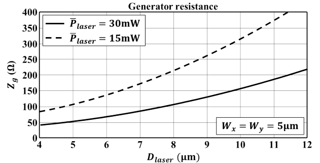
Figure 4. Laser beam diameter dependency of the generator resistance of a photoconductor material illuminated by a laser operating in PW mode.
