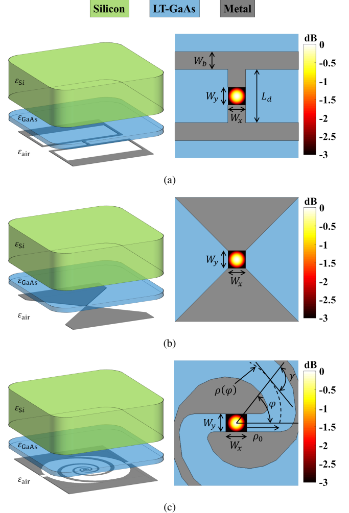
Figure 5. PCA geometries and structures: the blue slab represents the chip of photoconductive material; the green thick slab depicts the silicon semi-infinite medium; whereas the antenna metallizations are depicted in grey. a) H-dipole antenna: gap size W_x = W_y = 10 \mu\text{m} , dipole length L_d = 30 \mu\text{m} and bias lines width W_b = 10 \mu\text{m} . b) Bow-tie antenna: gap size W_x = W_y = 10 \mu\text{m} and tapering angle 90^\circ . c) Logarithmic spiral antenna: \rho(\varphi) = \rho_0 e^{a\varphi} with \varphi \in [0, 2\pi N] , starting radius \rho_0 = 23 \mu\text{m} , curvature angle \gamma = 76.5^\circ , winding number N = 2.6 , tapering angle \delta = 150^\circ and gap width W_y = 10 \mu\text{m} . In the zoom of the gap of each antenna, it is shown the normalized laser power density spatial distributions, D_{laser} = 10 \mu\text{m} , used for the evaluation of the energy spectral density in Fig. 7.
