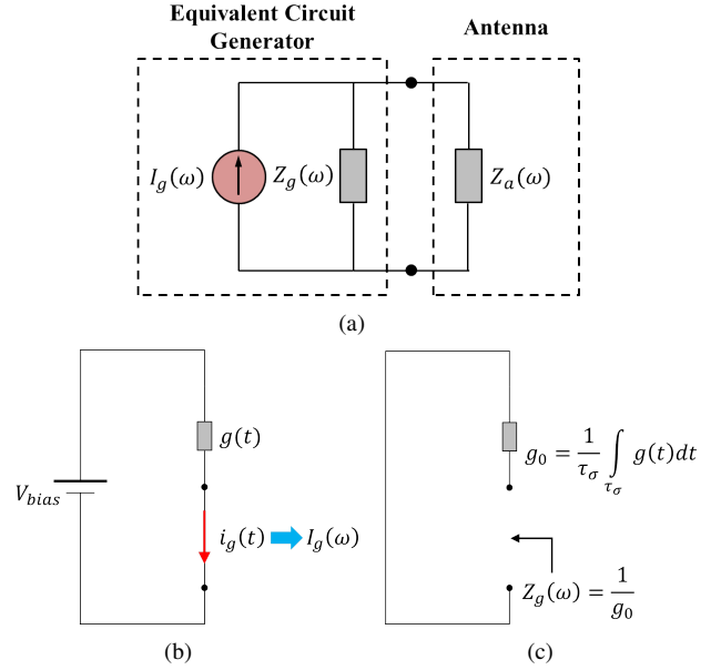
Figure 2. a) Equivalent Norton frequency-domain circuit. Schematic derivation for b) the equivalent generator current, and c) the equivalent generator impedance.
