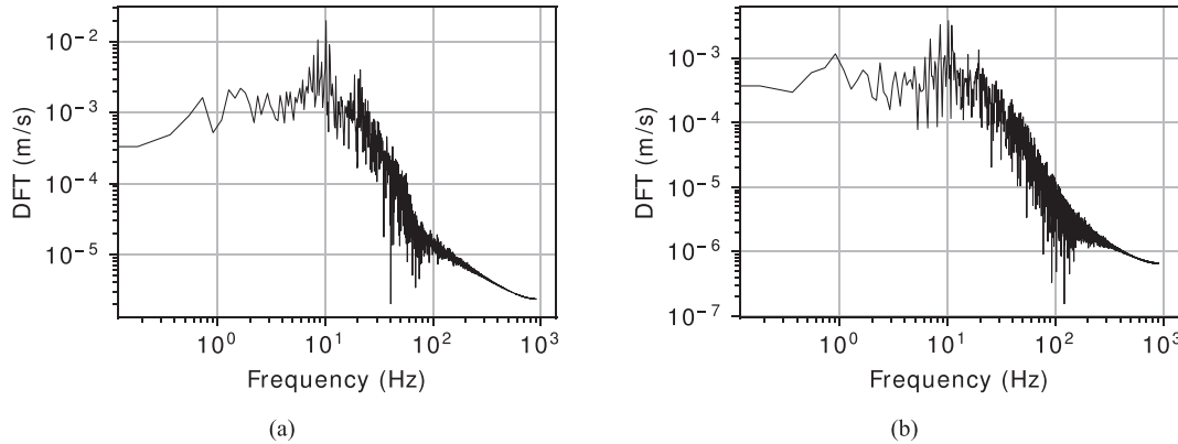
Fig. 8. Magnitude of the Discrete Fourier transform of (a) the radial velocity component at the 5th point from the central rod for Q = 2.141/s and (b) the axial velocity component at the 8th point from the central rod for Q = 2.141/s .
