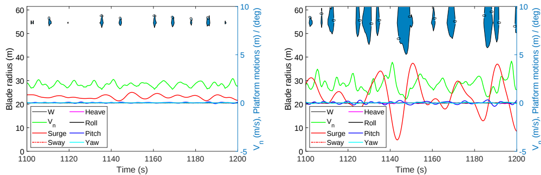
Figure 3. TLP with normal irregular waves (LC1)
