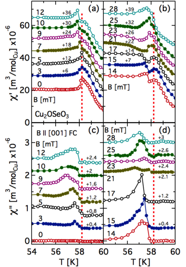
FIG. 4. Temperature dependence of FC \chi' (a),(b) and \chi'' (c),(d) for different magnetic fields B and for f = 0.8 Hz. The vertical dashed lines indicate T_c for B = 0 . For the sake of clarity the curves have been shifted vertically with respect to the base line by the numbers given next to each of them.
