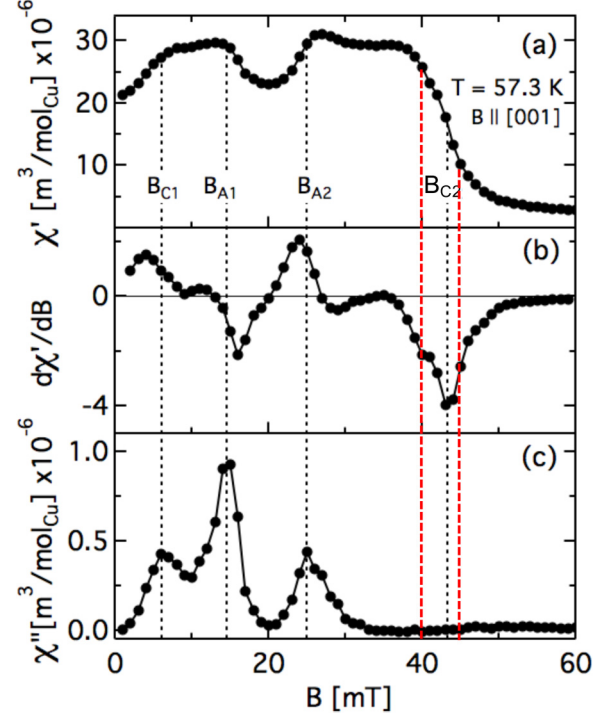
FIG. 6. Magnetic-field dependence of ZFC \chi' , its derivative d\chi'/dB , and the corresponding \chi'' of \text{Cu}_2\text{OSeO}_3 at T = 57.3 K for B \parallel [001] and f = 0.8 Hz. The maxima of \chi'' define the lower critical field B_{C1} = 6 mT as well as the lower and upper boundaries of the A phase, B_{A1} = 14.5 mT and B_{A2} = 25 mT, respectively. The upper critical field ( B_{C2} = 43 mT) was determined from the inflection points of \chi' and the extrema of d\chi'/dB . The red dotted lines correspond to the inflection points of d\chi'/dB at the two sides of B_{C2} and thus to the lower and upper boundaries of this transition. The unit of d\chi'/dB is \text{m}^3/(\text{mol}_{\text{Cu}} \text{mT}) \times 10^{-6} .
