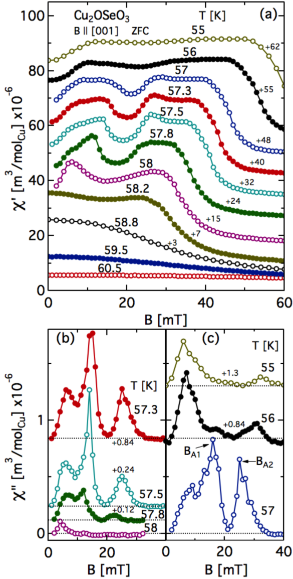
FIG. 5. Magnetic-field dependence of ZFC \chi' (a) and \chi'' (b), (c) of \text{Cu}_2\text{OSeO}_3 for some selected temperatures and for f = 0.8 Hz. For the sake of clarity some curves have been vertically shifted with respect to the base line by the values indicated next to each of them.
