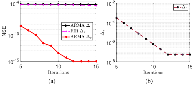
Fig. 2. (a) NSE between the quantized output and the unquantized output of FIR and ARMA filtering over time-invariant graphs for the Tikhonov denoising problem, where N = 10000 , a_s = 2200 m, \mathbf{S} = \lambda_{\max}^{-1} \mathbf{L} and w = 0.3 , \psi_{\max} \lambda_{\max} = 0.3 . The FIR filter coefficients are optimized by solving (15), with \Delta_0 = 0.15 and \chi = 25 bits. The x-axis is the number of iterations for the ARMA 1 filter, while for the FIR filter “Iterations = K ”. (b) Decreasing quantization stepsize over iterations is given by \Delta_\tau = (0.3)^t \Delta_0 for b_\tau \leq \chi .
