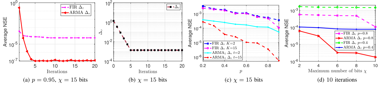
Fig. 4. (a), (c), and (d) Average NSE between the quantized output over time-varying graph and the unquantized output over a deterministic graph for both FIR and ARMA filters for the Tikhonov denoising problem, where N = 10000 , a_s = 2200 m, \mathbf{S} = \lambda_{\max}^{-1} \mathbf{L} , w = 0.25 , \Delta_0 = 1.36 and \psi_{\max} \rho = 0.25 . The FIR filter coefficients are optimized by solving (32). (a) Average NSE vs. iterations, where p = 0.95 and \chi = 15 bits. The x-axis is the number of iterations for the ARMA 1 filter, while for the FIR filter “Iterations = K ”. (b) Decreasing quantization stepsize over iterations is given by \Delta_\tau = (0.25)^\tau \Delta_0 for b_\tau \leq \chi . (c) Average NSE vs. the probability p of link activation, where \chi = 15 bits. (d) Average NSE vs. the maximum number of bits \chi at each iteration, where K = 10 for FIR filter and t = 10 for ARMA 1 filter.
