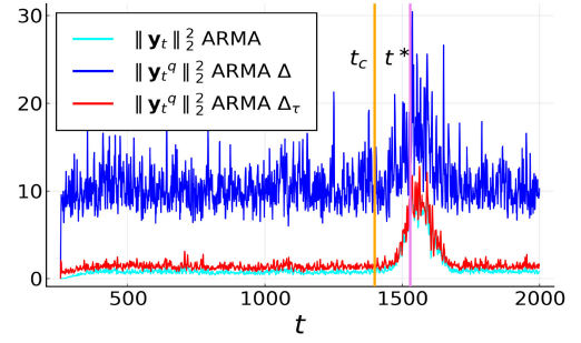
Fig. 3. Squared norm of unquantized and quantized filtered streaming graph signals for the change point detection problem, when using the ARMA 4 filter of NOUGAT algorithm [53], where N = 200 , a_s = 300 m, \mathbf{S} = \mathbf{L}_n - \mathbf{I} , \Delta_0 = 1.19 , \chi = 5 bits. The change-point is set at t_c = 1400 and the NOUGAT detection is expected at t^* = t_c + 128 for the same NOUGAT parameter values of [53].
