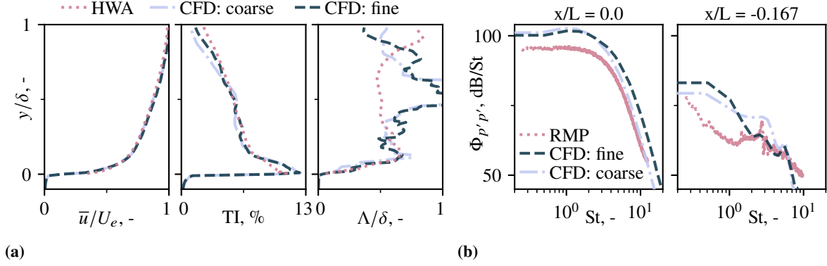
Fig. 5 Comparison between wind-tunnel measurements (HWA and WPS) and simulation data with the standard, i.e., fine , and the coarse mesh. The conditions are d_c = 4.5 mm and U_e = 15 m s -1 . (a) Boundary-layer profiles for x/L = 0 ; (b) WPS on the upper ( x/L = 0 ) and lower surface ( x/L = -0.167 ) of the porous wall-insert.
