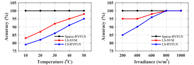
Fig. 4. Comparison of OC fault detection accuracy by Sparse-RVFLN, LS-SVM, and LS-RVFLN.
