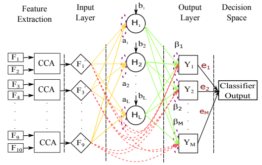
Fig. 1. CCA based RVFLN's structure.
