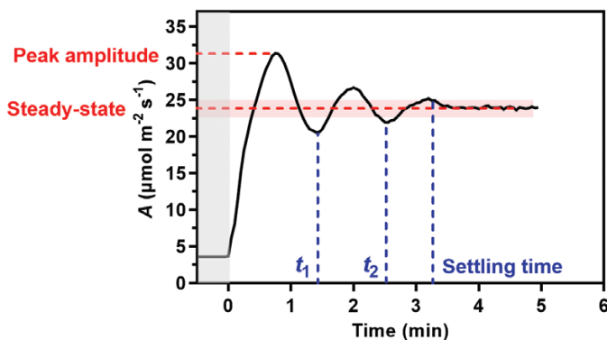
Fig. 1. Example of damped photosynthetic oscillation in a tomato leaf after an increase from a low light intensity ( 50 \mu\text{mol m}^{-2} \text{s}^{-1} ; shaded area) to a high light intensity ( 1000 \mu\text{mol m}^{-2} \text{s}^{-1} ; at time=0) under saturating CO_2 concentration. Key oscillatory parameters derived from the curve are shown, including peak amplitude, steady-state value, and settling time. Settling time is reached when photosynthetic rate ( A ) has fallen to within \pm 5\% (indicated as the light red bars) of the final steady-state value. t_1 and t_2 are the time of first and second trough.
