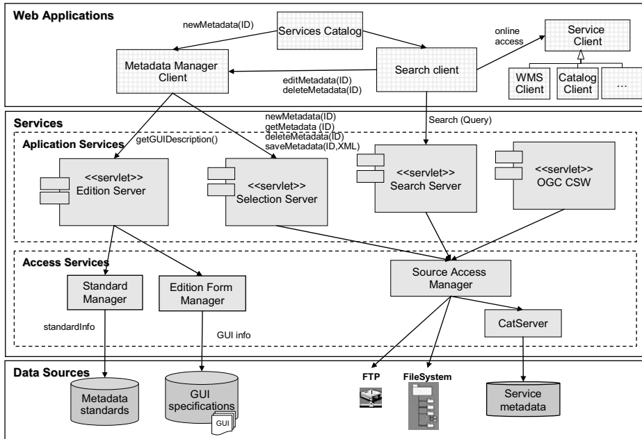
Figure 1: Services Catalog general architecture.
