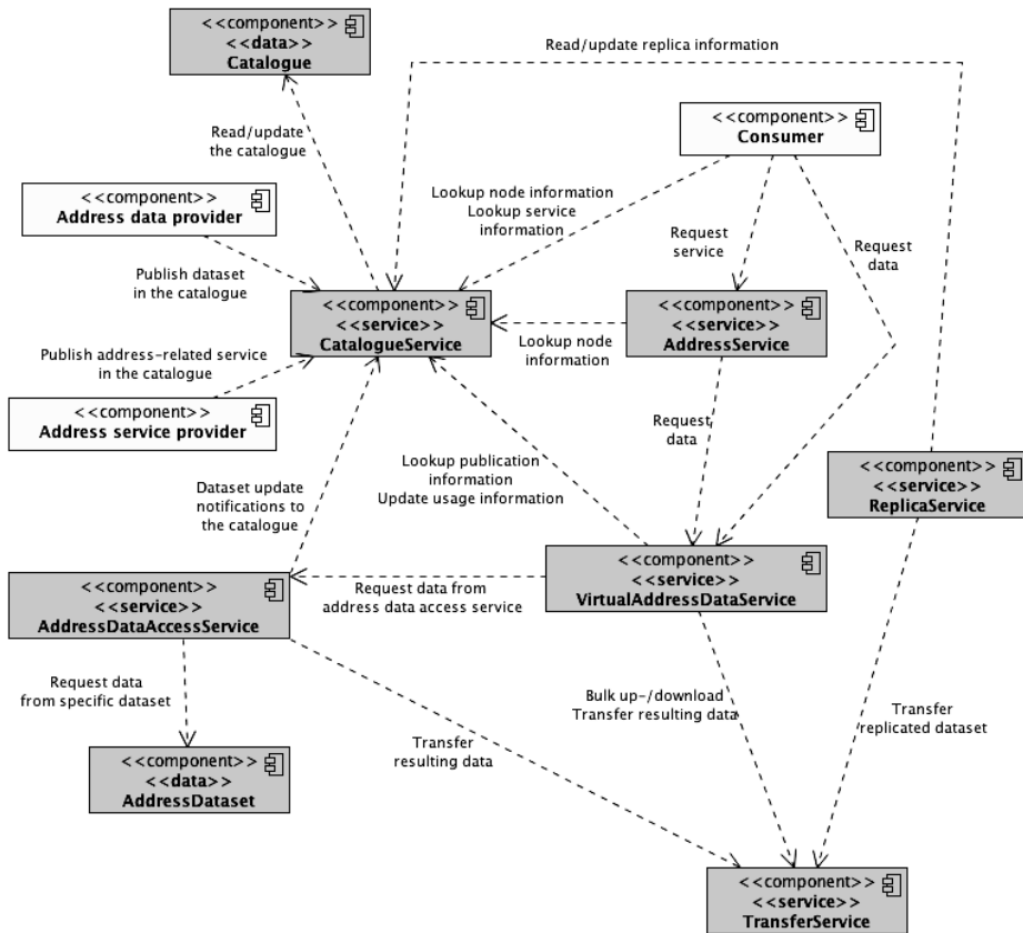
Figure 2: Object interaction in Compartimos.
