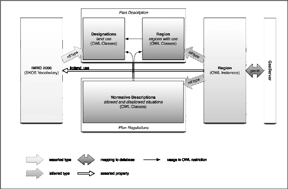
Figure 5: Conflict situation architecture.
