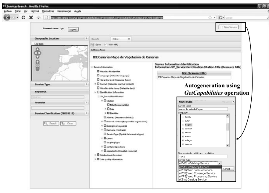
Figure 4: Online metadata edition.
