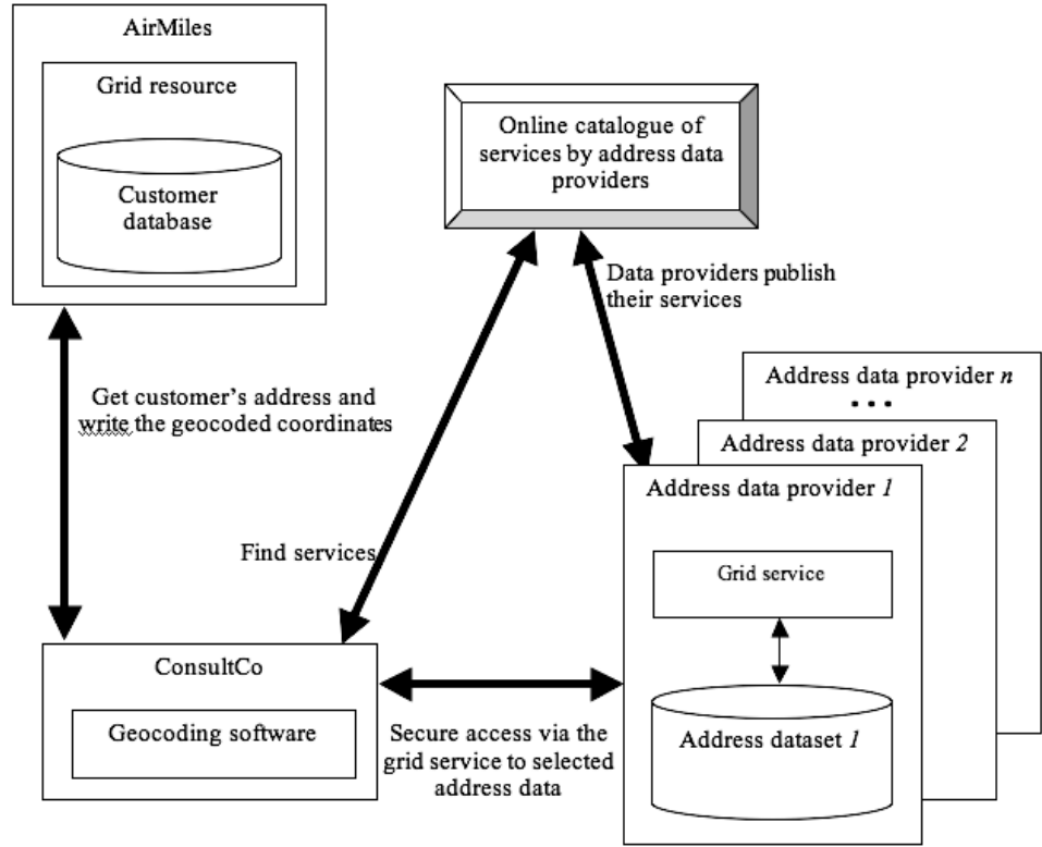
Figure 1: Geocoding a customer database.
