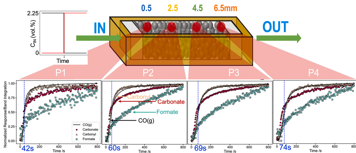
Fig. 5. Normalized surface species (scatter) and gas species (solid line) step responses after a switch from 2.25 vol% ^{12}\text{CO}_2/9\% H 2 → 2.25 vol% ^{13}\text{CO}_2/9\% H 2 /2.5 % Ar at 200 °C over a 3 wt% Pt/CeO 2 catalyst. Conditions: F = 50 mL/min, P = 1 bar, W_{\text{cat}} = 180 mg.
