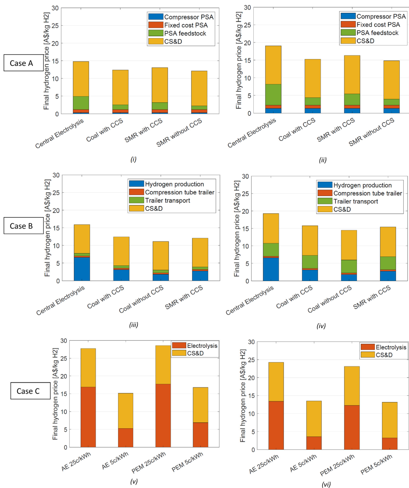
Fig. 9 – Cost break-down for the different hydrogen supply methods analysed. (i) Best case and (ii) worst case scenario for PSA supplied hydrogen at refuelling station. (iii) Best case and (iv) worst case scenario for tube-trailer delivered hydrogen at refuelling station. (v) Current and (vi) future prospected hydrogen price for onsite electrolysis at a refuelling station.
