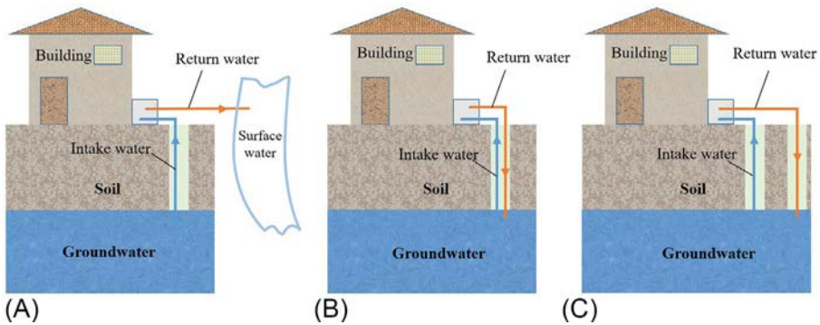
Fig. 8 The typical GWHP systems with different intake and return water modes: (A) Recharge to surface water; (B) Recharge to same well; (C) Recharge to different wells.
