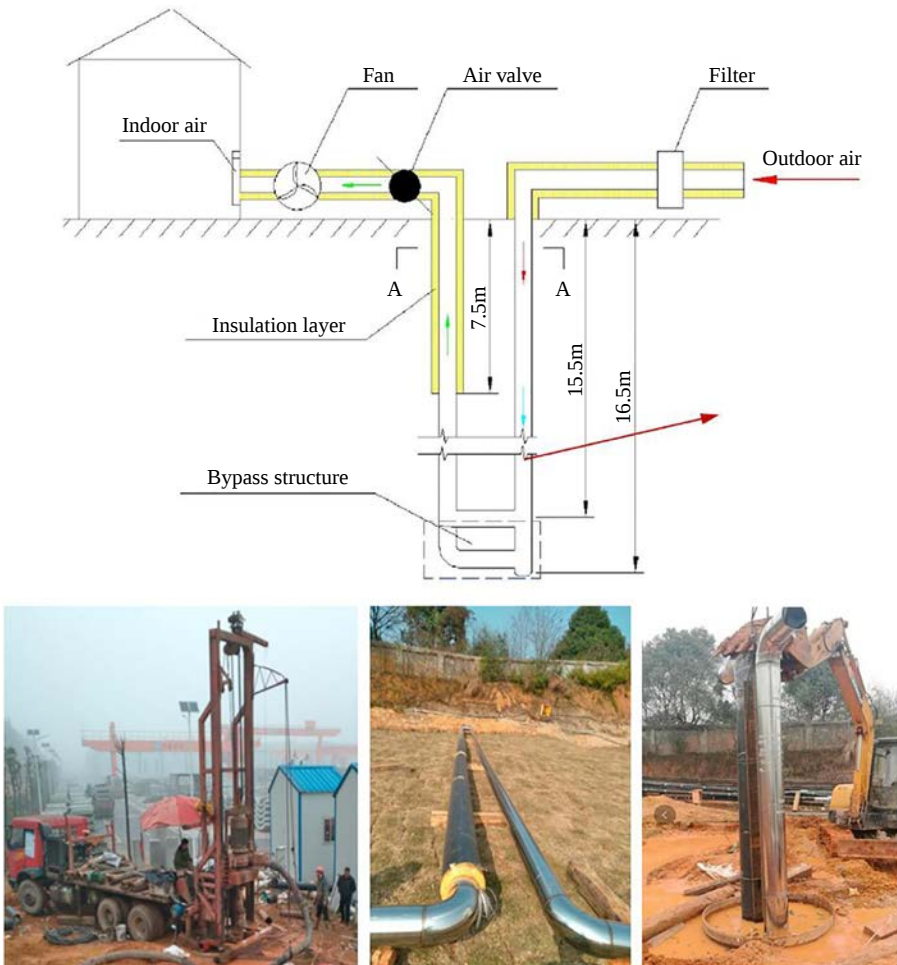
Fig. 12 The schematic diagrams and construction pictures of the vertical UDS system. Reprinted from Z. Liu, Z. Yu, T. Yang, L. Roccamena, P. Sun, S. Li, et al., Numerical modeling and parametric study of a vertical earth-to-air heat exchanger system, Energy 172 (2019) 220–231. Copyright with permission from Elsevier.
