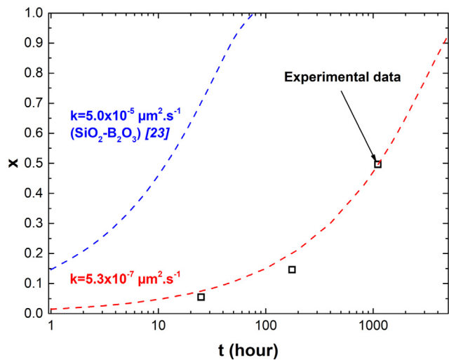
Fig. 9. Evolution of the oxidation ratio ( x ) of spherical \text{MoSi}_2 based particles as a function of time at a temperature of 1100 °C.
