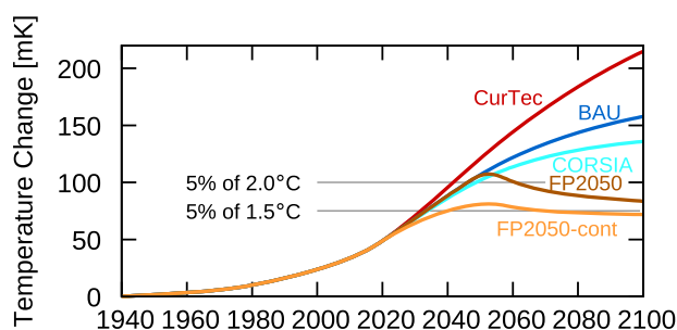
Fig. 2 Near-surface temperature change of five scenarios including CO 2 and non-CO 2 -effects. The horizontal lines indicate 5% of a 2 °C and 1.5 °C climate target. The scenarios describe a future use of current technology, i.e. without technology improvements (CurTec, red), a business-as-usual future technological improvement (BAU, blue), the offsetting scheme of the international civil aviation organisation (CORSIA, light blue), and 2 Flightpath 2050 scenarios which differ in the speed of technology improvements (FP2050 and FP2050-cont, brown and orange, respectively).
