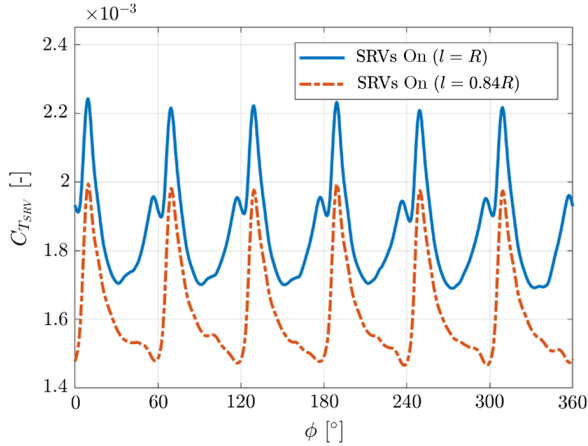
Fig. 20 Thrust coefficient of single vane C_{T_{SRV}} as a function of the phase angle \phi for a propeller rotation for the long and short vane configurations.
