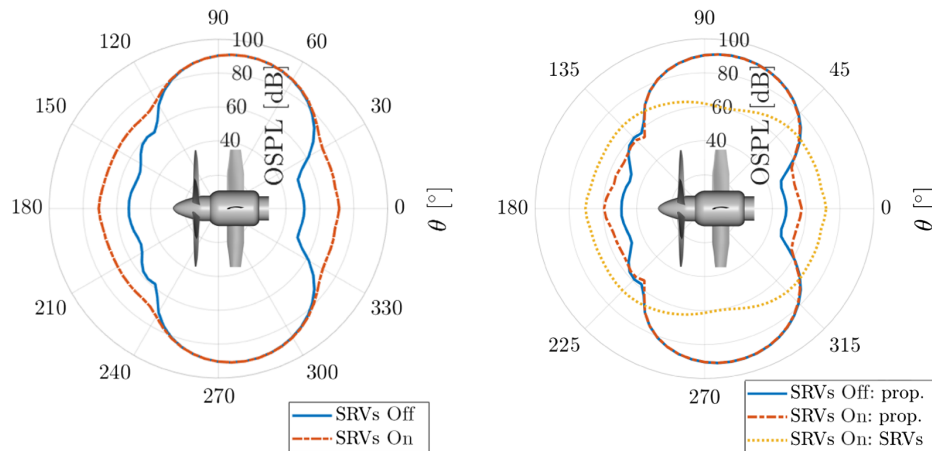
Fig. 16 Directivity plot of the OSPL computed on a sphere of radius 20R and centered at x/D = 0.2 . Data are plotted for both the SRVs on and off cases and are integrated between 0.5 BPF and 10 BPF. (Left) Full propulsive system and (right) separate contribution of each component.
