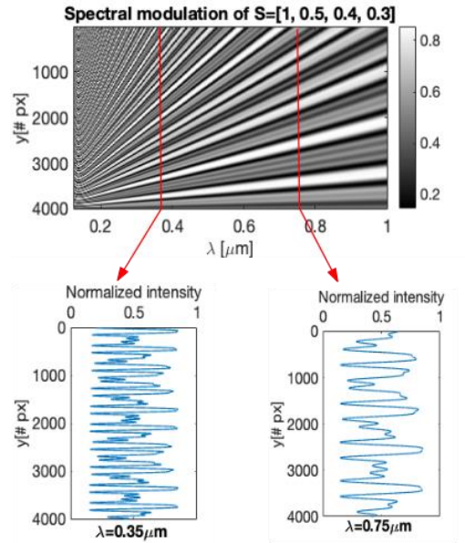
Figure 3-2. Spectral modulation of an incoming state of polarisation S=[1, 0.5, 0.4, 0.3] obtained on a column of 4000 pixels, with a size of 5\mu\text{m} . In this simulation we supposed that the height of modulator is h=2\text{cm} , the apex angles are \xi=2.6^\circ, \psi=1.8^\circ , and the additional thickness is d=1\text{mm} . The orientation of the analyser was \theta=72^\circ .
