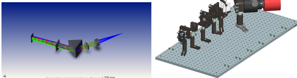
Figure 4-1. Left: Impression of the optical design of the spectropolarimeter. The incoming light is on the right, the detector on the left. Right: Rendered image of the optical and mechanical parts of the breadboard spectropolarimeter. Light enters on the left; the detector is mounted in the red cylinder on the right.
