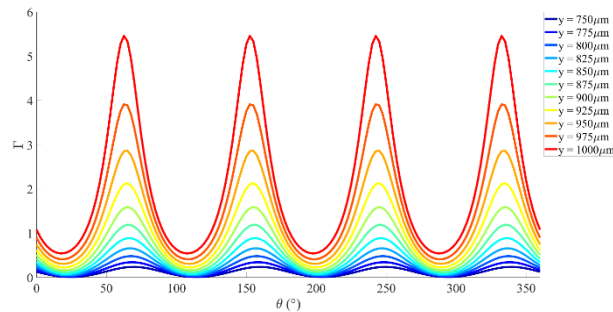
Figure 5-2. Representation of the intensities ratio \Gamma for pixels on the same column and at different height inside the modulator. The representation step was selected as 25\mu\text{m} to provide more variation with fewer curves. The real system will be on the 5\mu\text{m} range for the pixel size.
