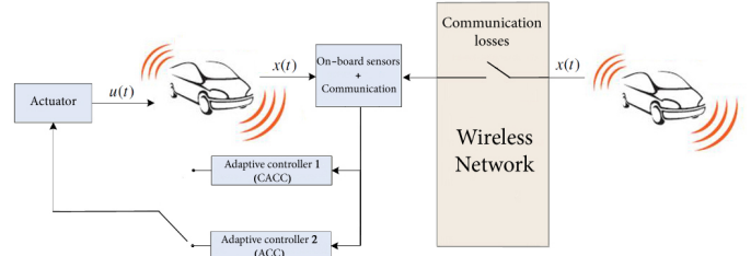
Fig. 2. Networked switched control system
