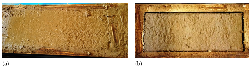
Figure 7.5: Shrinkage of mortar after five days of curing (a): volumetric shrinkage of 18% (b)
