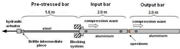
Figure 4.2: Setup of servo-hydraulic machine tests (a); Detail of Hopkinson bar in front of the specimen (b); Schematic picture of the JRC modified Hopkinson test setup for compression (c)
