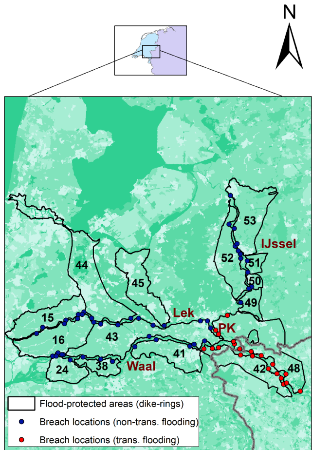
Figure 5.1 Transboundary case study area with the grey line representing the administrative border. Black thick lines represent dike-rings, i.e. dike-protected areas, with the code relative to each dike-ring reported within. Dots are breaching locations, with flooding at the red dots causing transboundary damage, i.e. damage in both countries. Beside the German Rhine, four branches are identified: Boven-Rijn (downstream the German Rhine, up to the bifurcation point), Waal, Pannerdensch-Kanaal (PK in the map), the Lek and the IJssel.
