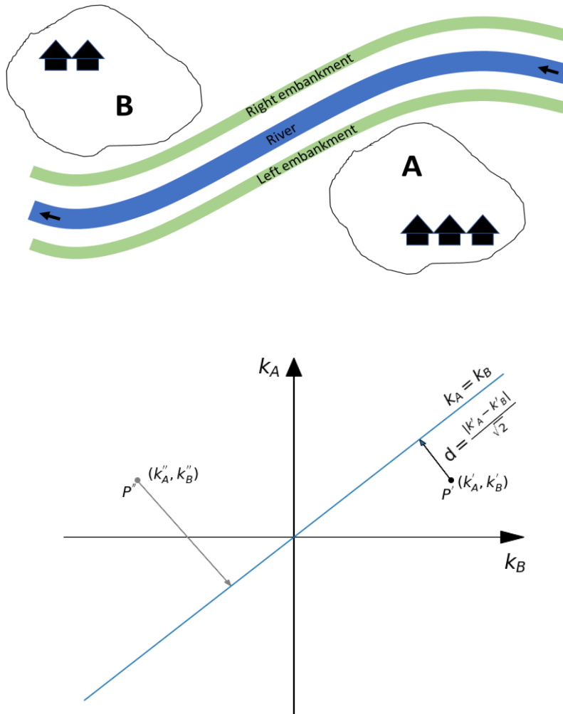
Figure 3.11 Top: Stylized representation of a flood risk system with two flood protected areas, A and B. Bottom: visualization of the geometric approach used to quantify the distribution of benefits among areas. The axes represent the outcome indicator of area A, k_A , and area B, k_B . The bisector is the line of equal benefits, i.e. a condition where area A and B have the same k . Points P' and P'' indicate the effect of two distinct policies on the outcome indicators. The distance d indicates the geometric distance between a point to the bisector line, i.e. d indicates how far the distribution of benefits brought by a given policy is from an equal distribution.
