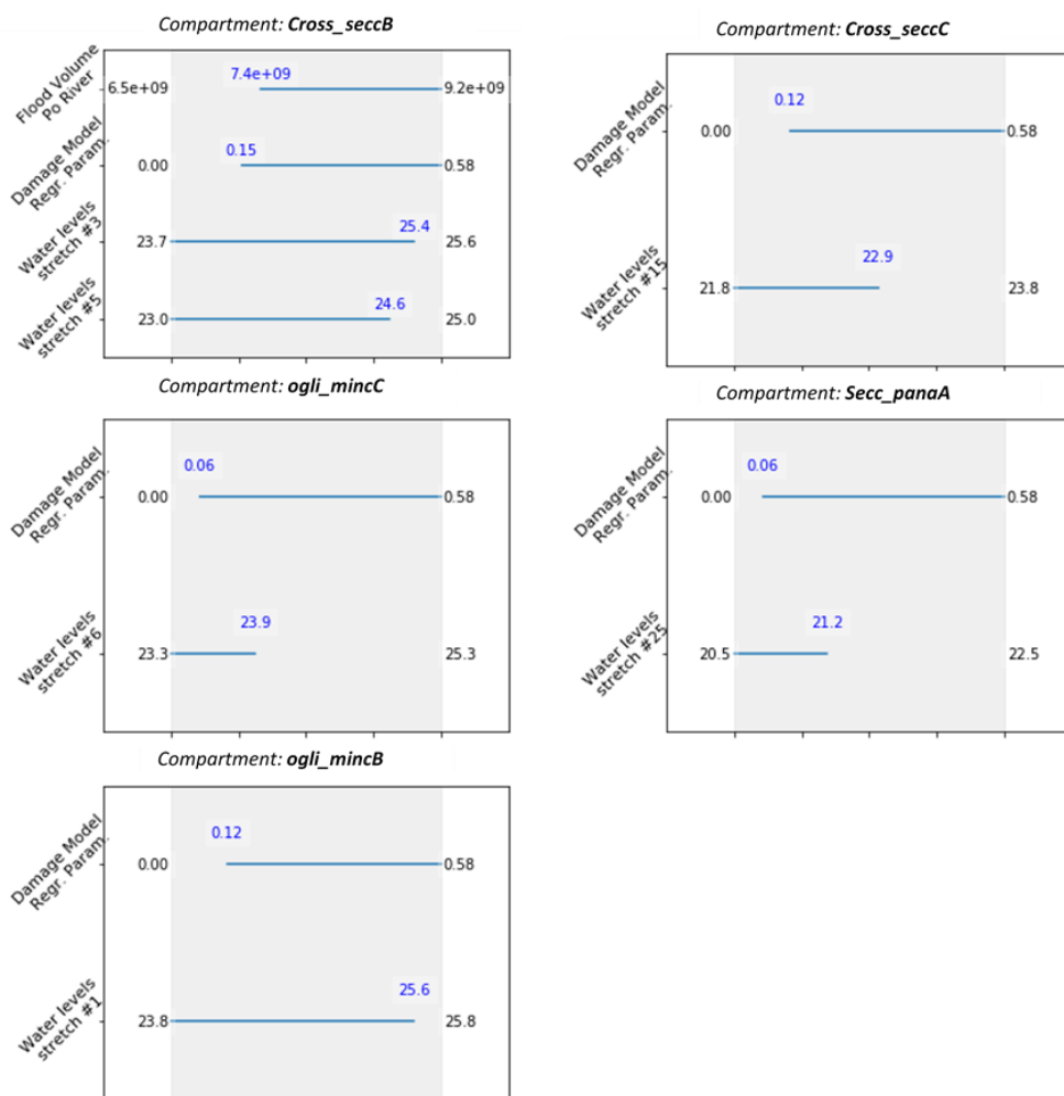
Figure 4.9 Scenario Discovery results. Uncertain parameters and value ranges leading each compartment to flood damage higher than the 3 rd quartile. Flood volume is expressed in cubic meters, breaching water levels in meters above sea level and the damage model regression parameter is adimensional.
