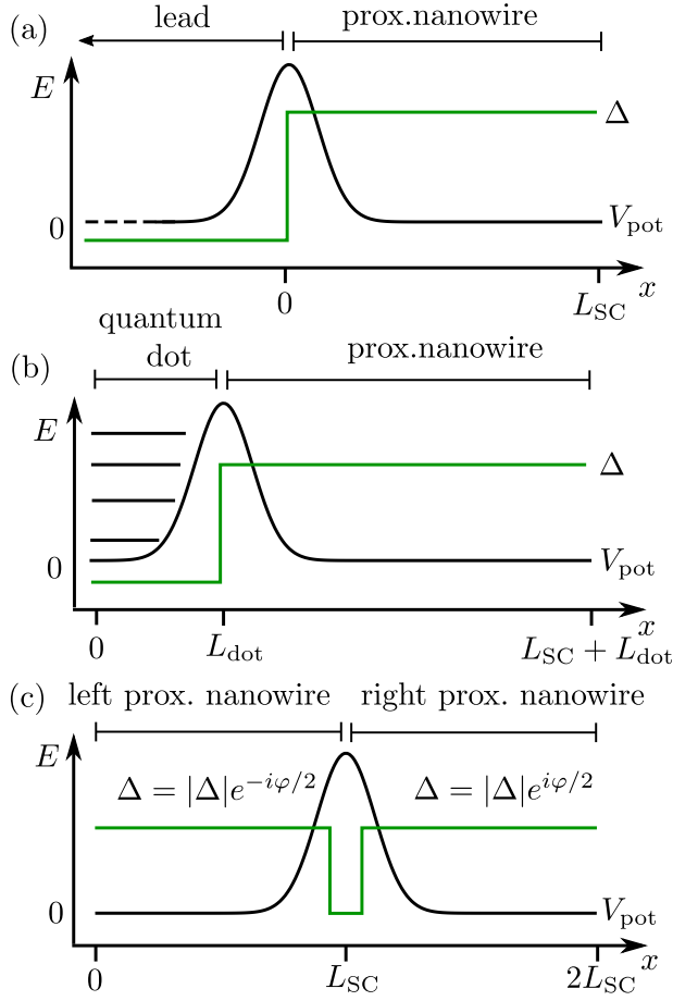
Figure 4.2: Schematic drawings of the three studied devices. The black lines indicate the potential profile V_{pot}(x) , the green lines the superconducting gap \Delta(x) . (a): Proximitized nanowire of length L_{SC} with constant superconducting gap \Delta connected to a semi-infinite normal lead from the left via a potential barrier. (b): Proximitized nanowire of length L_{SC} connected to a normal quantum dot of length L_{dot} on the left via a potential barrier V_{pot} . (c): Two finite proximitized nanowires, both of length L_{SC} , with a superconducting phase difference \varphi between them, and separated by a potential barrier V_{pot} .
