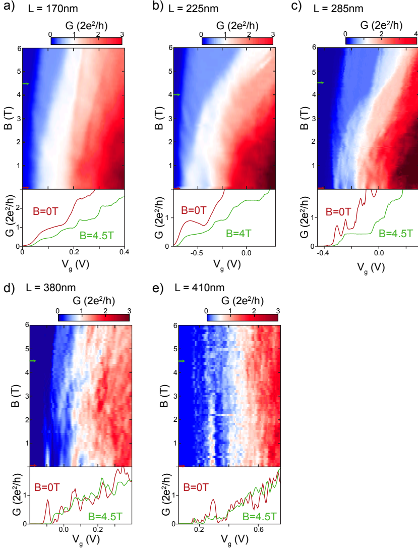
Figure 3.10: Length dependence of nanowire QPCs. Magneto-conductance measurements (at V_{SD} = 0 mV) of QPCs with increasing length. The contact spacing L is changed in steps of \sim 50 nm. (a)–(c) are shorter and (d,e) are longer than device 1 ( L = 325 nm). Line traces at 0 T and finite field are added in the bottom panel. The short channel devices (a, b) show well defined and flat plateaus throughout the full magnetic field range. For intermediate channel lengths, (c), resonances start to appear and modify the conductance at low magnetic fields. Long channel devices, (d, e), are dominated by backscattering and conductance fluctuations dominate for the full magnetic field range.
