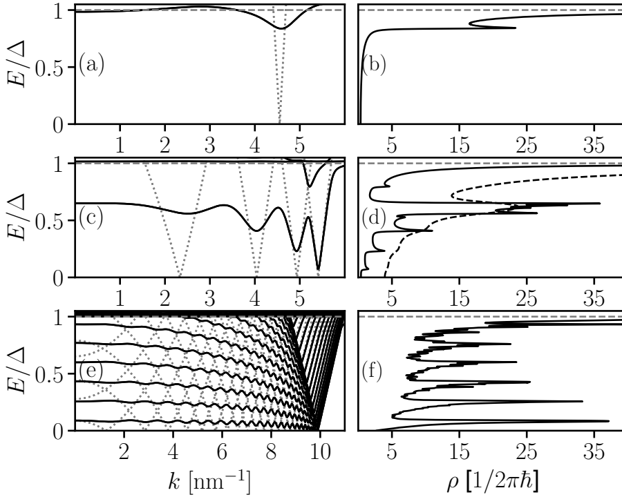
Figure 5.13: Dispersion (left column) and density of states (right column) of a quasi one-dimensional normal-superconductor junction in different regimes: a short junction (top), an intermediate junction (middle) and a long junction (bottom). In the left column, the dotted curves show the electron and hole dispersions of the corresponding normal channel with the superconductor removed. In all cases, a small broadening \Gamma \ll \Delta has been added to the density of states. For the intermediate junction (d), the density of states with larger broadening is also shown (dashed curve). The curves are symmetric under (k, E) \rightarrow (\pm k, \pm E) .
