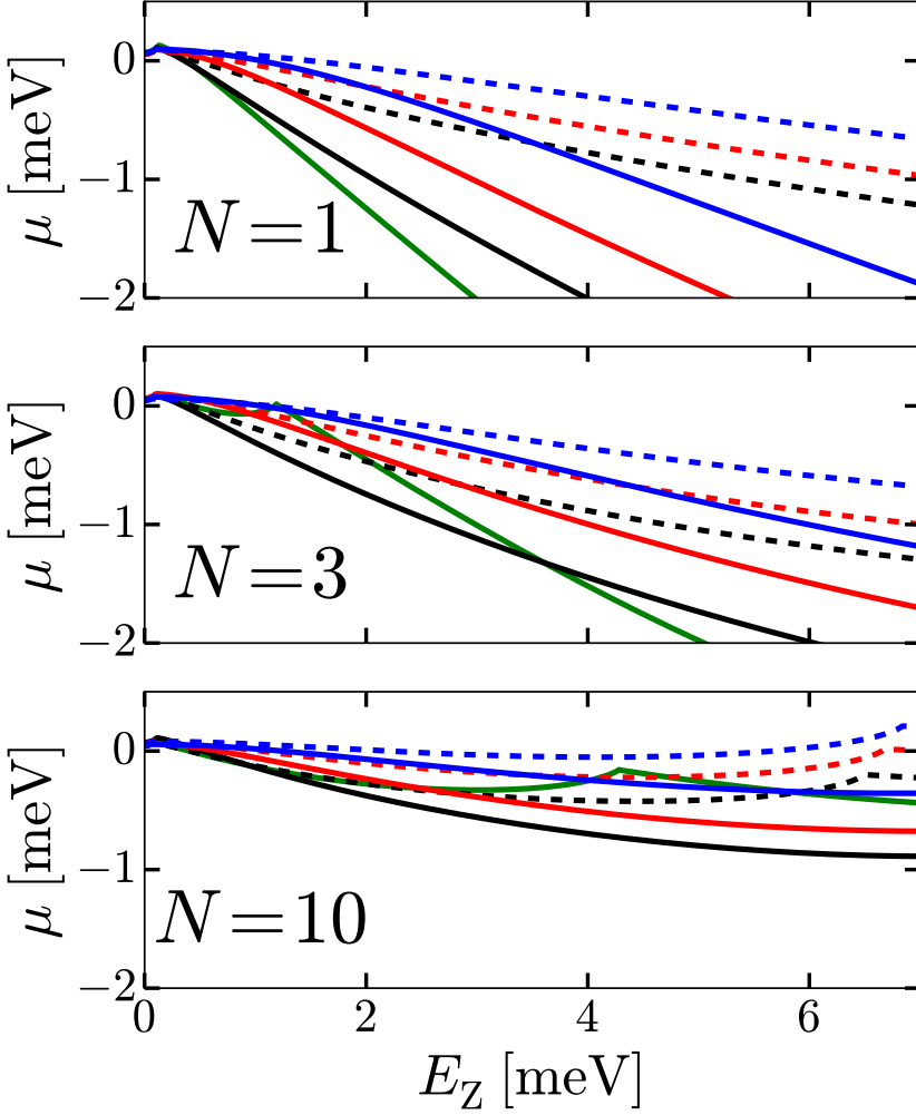
Figure 2.6: Response of \mu_N as a function of magnetic field for N = 1, 3 , and 10 , all close to the band bottom. The solid green line corresponds to the case of no screening by a superconductor. Other solid lines correspond to V_{SC} = 0 V, dashed lines to V_{SC} = 0.2 V. Black, red and blue indicate spin-orbit lengths of 233, 100, and 60 nm respectively.
