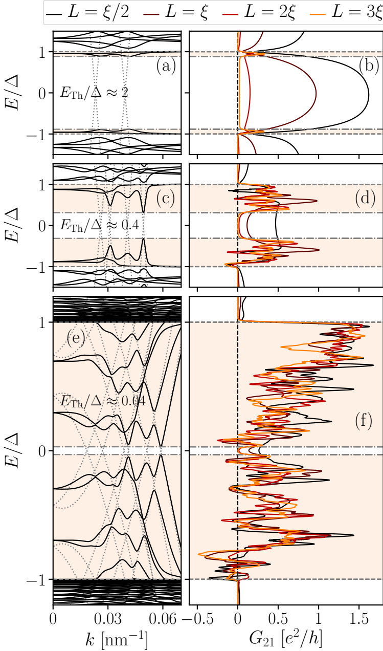
Figure 5.5: (a, c, e) Dispersions of proximitised systems that are translationally invariant along x , and (b, d, f) nonlocal conductance G_{21}(E) of corresponding junctions of finite length. The latter is shown as the separation L between the two normal leads is varied, with brightening colors from black to orange denoting L = \xi/2, \xi, 2\xi and 3\xi , respectively. The ratio E_{\text{Th}}/\Delta becomes smaller from top to bottom, such that \Delta_{\text{ind}} shrinks (dash-dotted lines). For L \gg \xi , the nonlocal conductance is suppressed if |E| < \Delta_{\text{ind}} , and finite only for \Delta_{\text{ind}} < |E| < \Delta (colored region). The solid lines in the dispersion relations show the dispersion of the normal-superconductor system, while the dotted lines show the electron and hole dispersion of the normal channel only, with the superconductor removed. We have W = 100 nm in (a) and (b), W = 200 nm in (c), (d), (e) and (f), and W_L = 100 nm always in the right column. \mu = 3 meV, \Delta = 0.2 meV and T = 30 mK in the top and middle rows, but \mu = 4.2 meV, \Delta = 2 meV and T = 100 mK in the bottom row. Dispersions are even in k .
