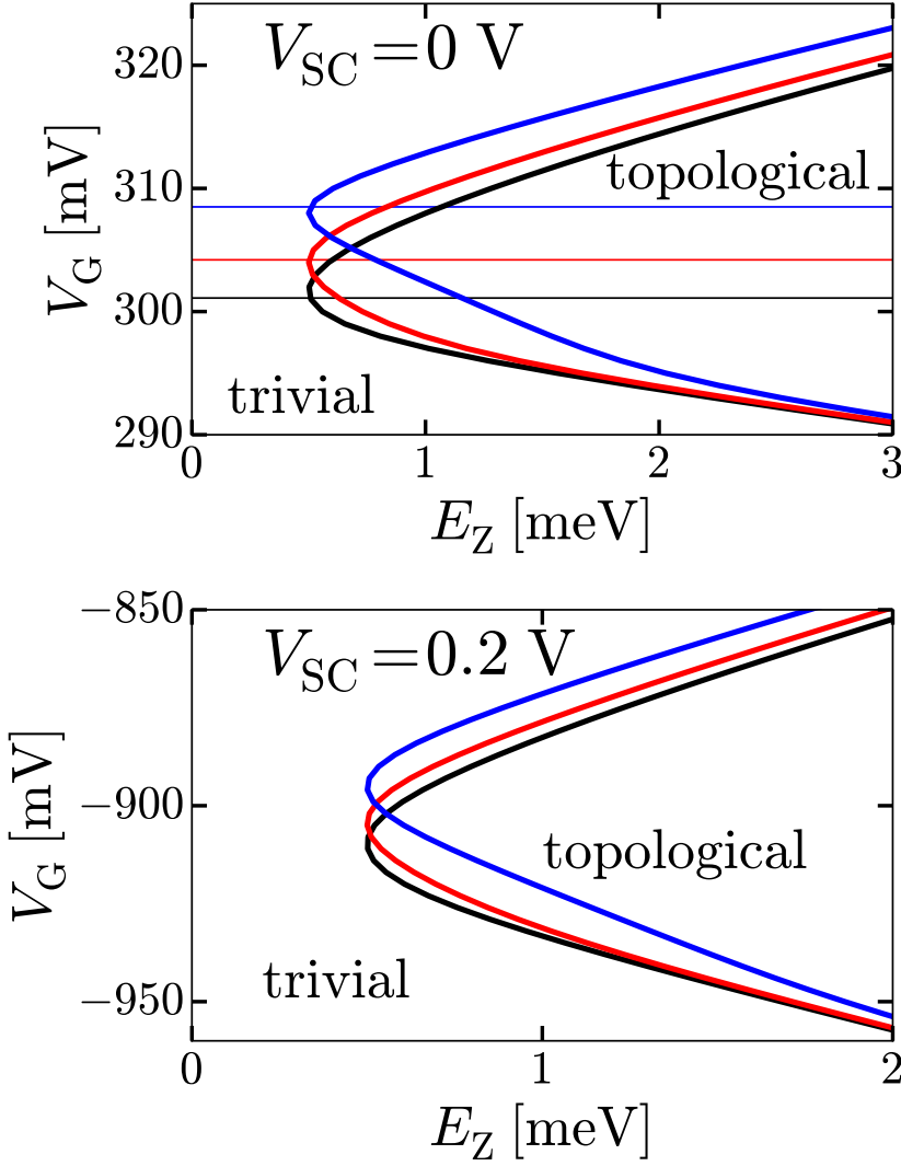
Figure 2.7: Majorana transition boundary for a superconductor at V_{SC} = 0 V (upper panel) or a superconductor at V_{SC} = 0.2 V (lower panel). The superconducting gap \Delta = 0.5 meV. The boundaries are obtained for the single-band case. The solid black, red, and blue lines correspond to a spin-orbit length of 233, 100, and 60 nm respectively. The black, red and blue horizontal lines in the upper plot indicate the gate voltages at which we compute the correspondingly colored Majorana coupling oscillations in the inset of Fig. 2.8.
