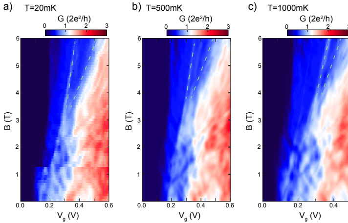
Figure 3.7: Temperature dependence of the helical gap. Measurements of the differential conductance dI/dV ( V_{SD} = 0\text{ mV} ) as function of magnetic field at (a): T = 20\text{ mK} (b): T = 500\text{ mK} (c): T = 1000\text{ mK} . The helical gap (dotted lines) evolves similarly in all three measurements showing that it stays stable at increased temperatures as expected for the energy scale extracted for E_{SO} .
