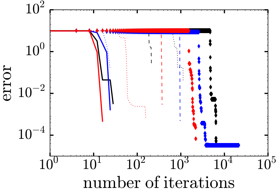
Figure 2.13: Benchmark of the Anderson solver (solid lines) with the First Broyden's method (dashed lines), the Second Broyden's method (dotted lines) and the BiCG-stab Newton-Krylov method (diamond markers). Black, blue and red colors correspond to a gate voltage V_G = 0.3, 0.4 , and 0.5 V respectively. We show the cumulative minimum of the error.
