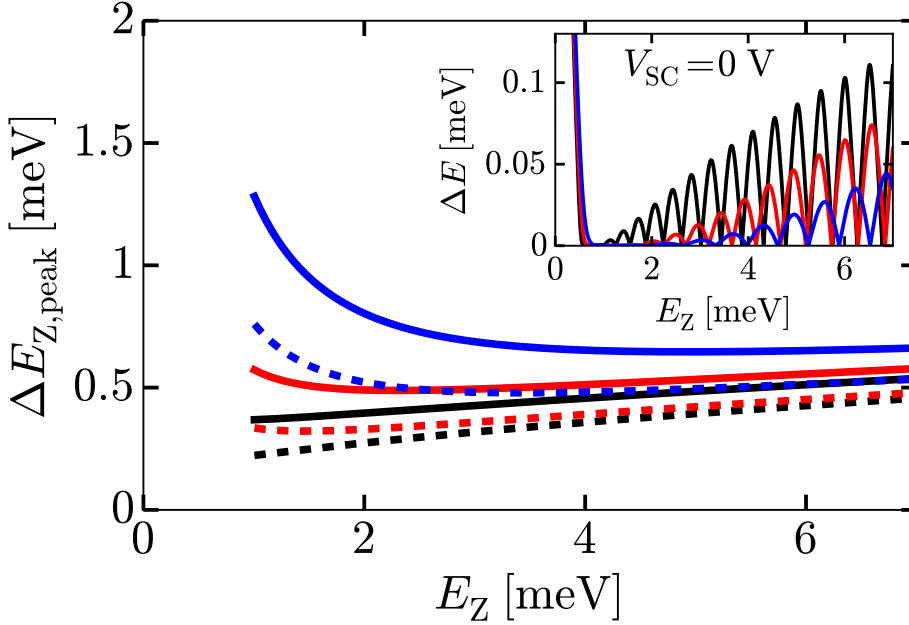
Figure 2.8: Peak spacing of the Majorana energy oscillations in a magnetic field for a nanowire of length L = 2\mu\text{m} . Solid lines correspond to V_{\text{SC}} = 0 V, dashed lines to V_{\text{SC}} = 0.2 V. Black, red and blue indicate spin-orbit lengths of 233, 100, and 60 nm respectively. Inset: Splitting energy oscillations for V_{\text{SC}} = 0 V. The three horizontal lines in the upper panel of Fig. 2.7 indicate the corresponding gate potential. The energy splittings are found by solving for the lowest energy of the Hamiltonian of Eq. (2.8), using the chemical potentials obtained from the perturbation scheme as described in Sec. 2.4.
