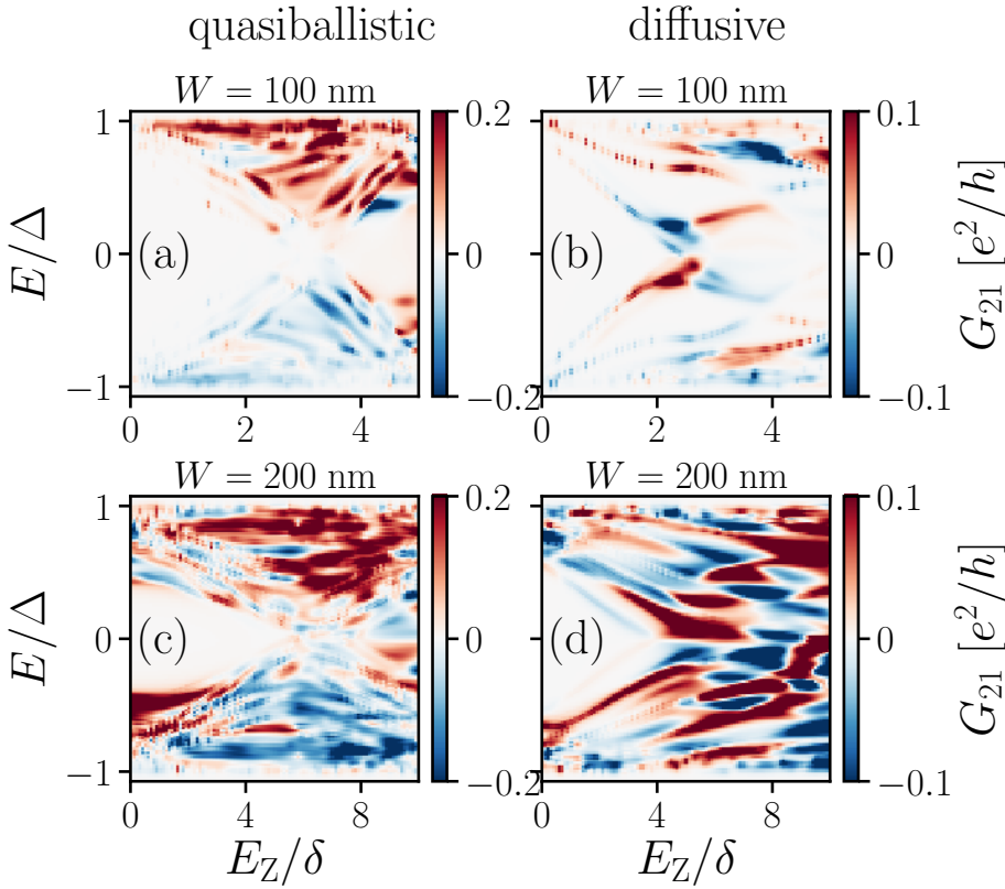
Figure 5.8: The nonlocal conductance G_{21} as a function of E and E_Z for a proximitised system that is quasiballistic (a, c with \mu = 3 meV) and diffusive (b, d with \mu = 16 meV). For the diffusive junction, the leads are gated into the single-mode regime using quantum point contacts at the junctions with the channel. Top and bottom row present results for W = 100 and 200 nm respectively. For the quasiballistic junction, L/\xi = 8 and 2 for W = 100 nm and 200 nm respectively, and the mean free path is l_e = 0.2L in each case. In the diffusive system, we have l_e = 0.2W and L/\xi = 5 and 2 for the widths respectively, where \tilde{\xi} = \sqrt{l_e \xi} . The color scale is saturated in both cases for clarity.
