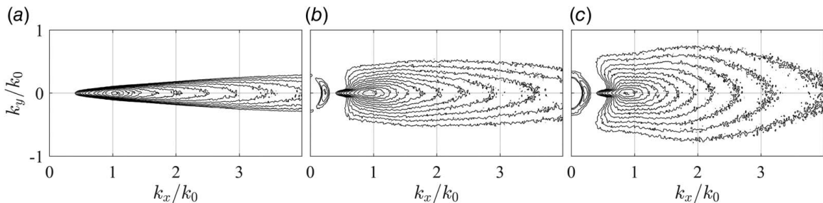
Fig. 4 Contour plots of the ensemble-averaged variance density spectrum \bar{S}(k_x, k_y) for case LT featuring truncation of the spectral tail in the vicinity of |k|/k_p = 6 : (a) t/T_0 = 0 , (b) t/T_0 = 50 , and (c) t/T_0 = 100 . The contour levels are logarithmic, ranging from 1 \times 10^{-5} to 1 \times 10^{-2} .
