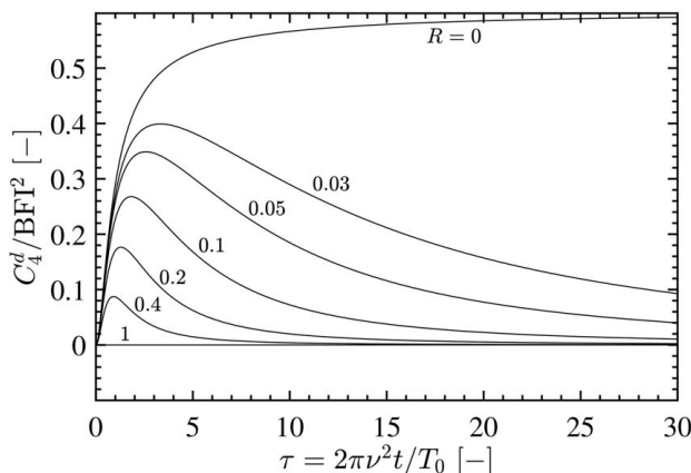
Fig. 1 Dynamic excess kurtosis normalized by the square of the Benjamin–Feir index ( C_4^d/BFI^2 ) as a function of nondimensional time ( \tau = v^2\omega_0 t ) for different values of R , based on Fedele [10]
