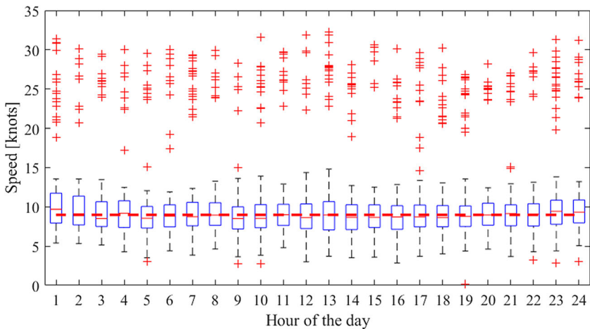
Figure 9. Vessel speeds per hour of the day (I2).
