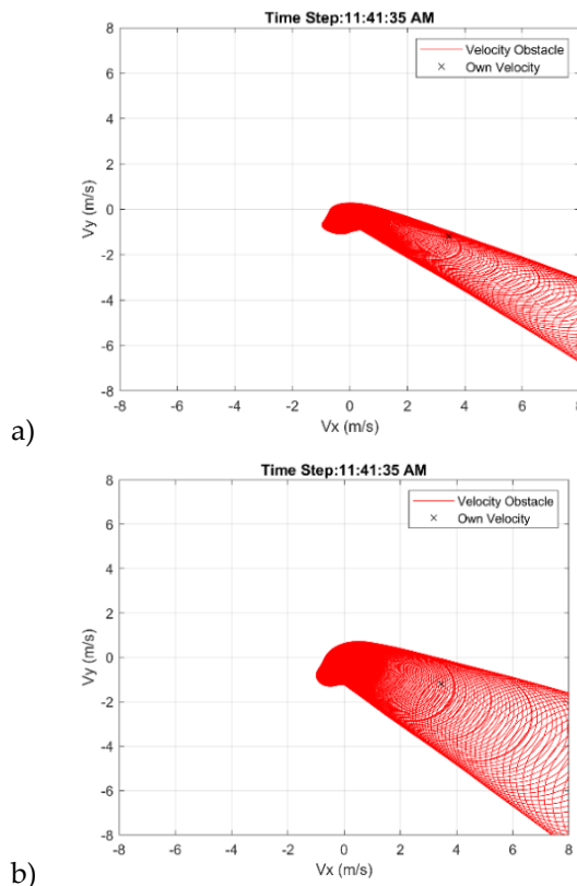
Figure 7. Illustration of Velocity obstacle obtained with M1 and M2 at 11:41:35 AM
