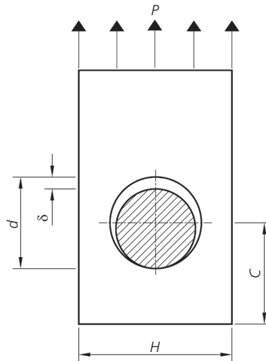
Figure 6.19 Provision for movement in point supported glazing panel. (Haldimann et al. , 2008.)
