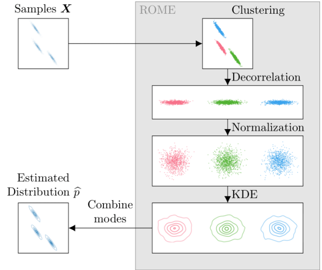
Figure 1: ROME takes samples from unknown distributions and estimates their densities to enable further downstream applications.
