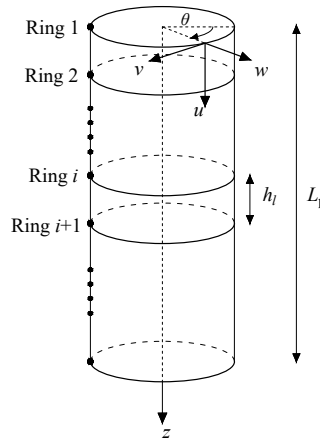
Figure 6.3: A thin cylindrical shell with axial discretization into nodal rings based on the SAFE method.
