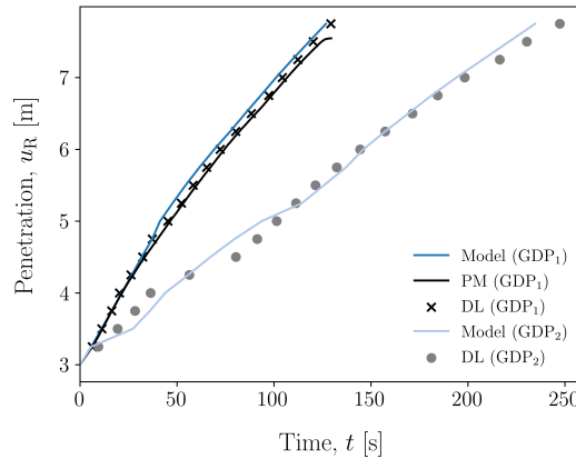
Figure 7.5: Comparison of GDP model predictions with field data for piles GDP 1 and GDP 2 ; penetration profiles as recorded both by the potentiometer (PM) and the vibratory device logging system (DL) are shown.
