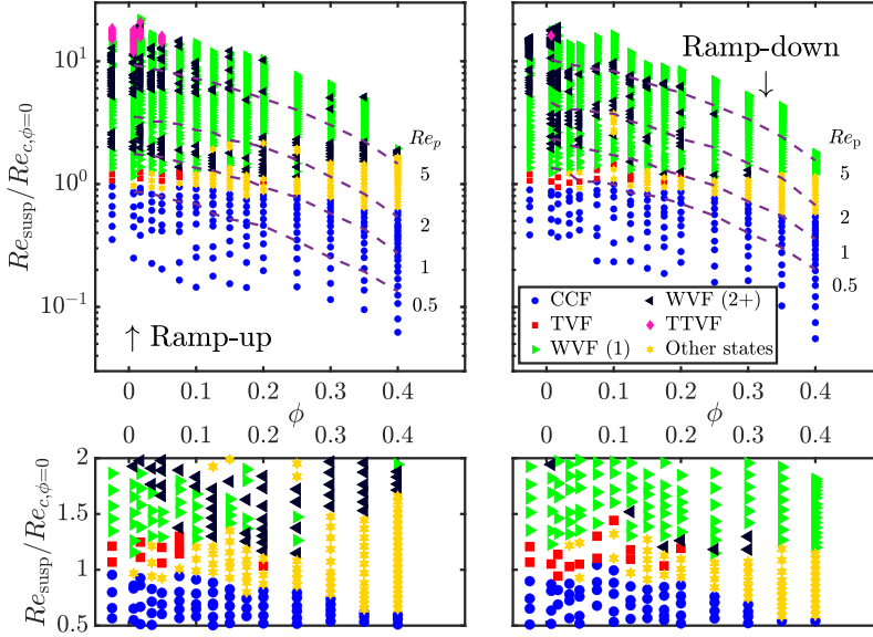
Figure 3.3: (Top) A consolidated regime map as a function of particle volume fraction as well as suspension Reynolds number (normalized by the experimentally determined critical Reynolds number for single-phase flows, Re_{c,\phi=0} = 142 ). In the legend, WVF (1) and WVF (2+) refer to periodic (single, distinct peak in the spectrum) and quasi-periodic (at least two, distinct, incommensurate peaks in the spectrum) wavy vortex flows, respectively. The single-phase flow case has been offset to aid better comparison. The purple dashed lines are approximate isolines for various particle Reynolds numbers. (Bottom) Zoomed-in portion of the consolidated regime map corresponding primarily to the lower-order transitions.
