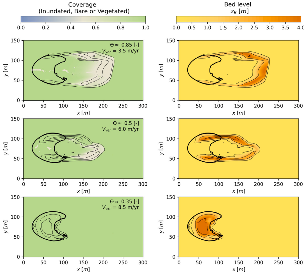
Fig. 8. Simulation overview of three simulated parabolic dunes for varying settings of fixation index ( \Theta \approx 0.85, 0.50 , and 0.35 [-]) by varying vegetation growth speed ( V_{\text{ver}} : 3.5, 6.0, and 8.5 m/year, resp.). See Video 2 for animated simulation results.
