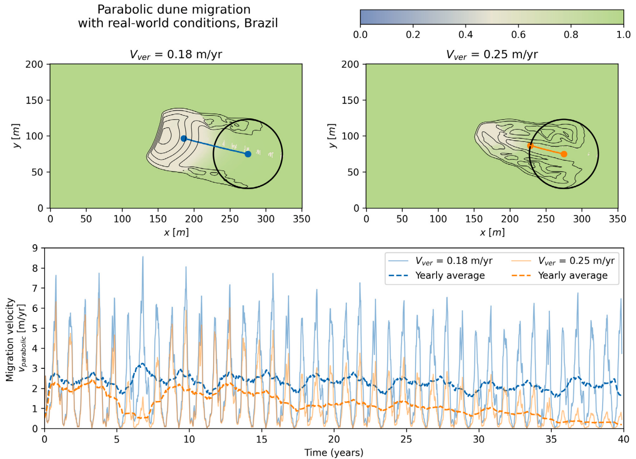
Fig. 9. Migration of parabolic dunes under real-world, Brazilian, wind conditions. The centre of both dunes is traced, as indicated by the blue and orange lines in the upper panels. The lower panel displays the monthly (continuous) and yearly (dotted) averaged migration rates for both simulations.
