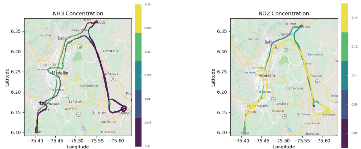
Figure 16. Simple space measurements of NH 3 and NO 2 over the Aburra Valley.
