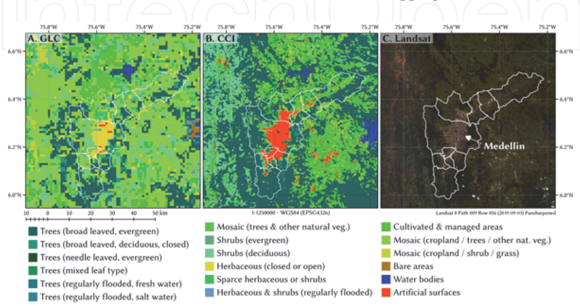
Figure 4. Comparison between (A) the LOTOS-EUROS's original land cover model (global land cover, with resolution of 1 km x 1 km.) and (B) the updated land cover scheme (land cover from the climate change initiative, with resolution 0.3 km x 0.3 km). Real color Landsat cloudless imagery for the date 2019-09-03 is included in (C) as a reference for the artificial surfaces from the city infrastructure. The political boundaries correspond to the municipality of Medellín and the other nine municipalities that constitute the Aburrá Valley metropolitan area conurbation.
