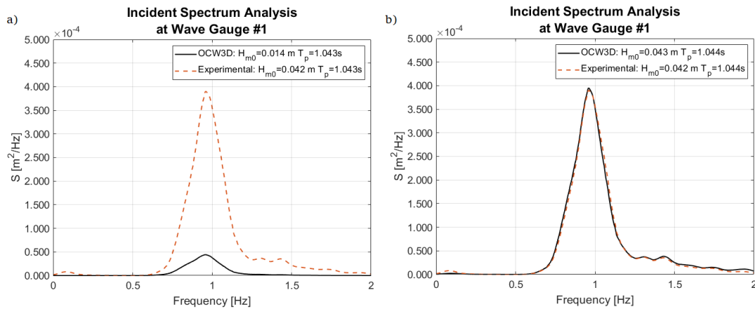
Figure 4. Comparison of incident Spectrum Analysis and water surface elevation at Wave Gauge 1 for operational conditions. a) Linear interpolation of the wave paddle data, b) FFT signal reconstruction of the wave paddle data. The numerical results are extracted from OCW3D domain.
