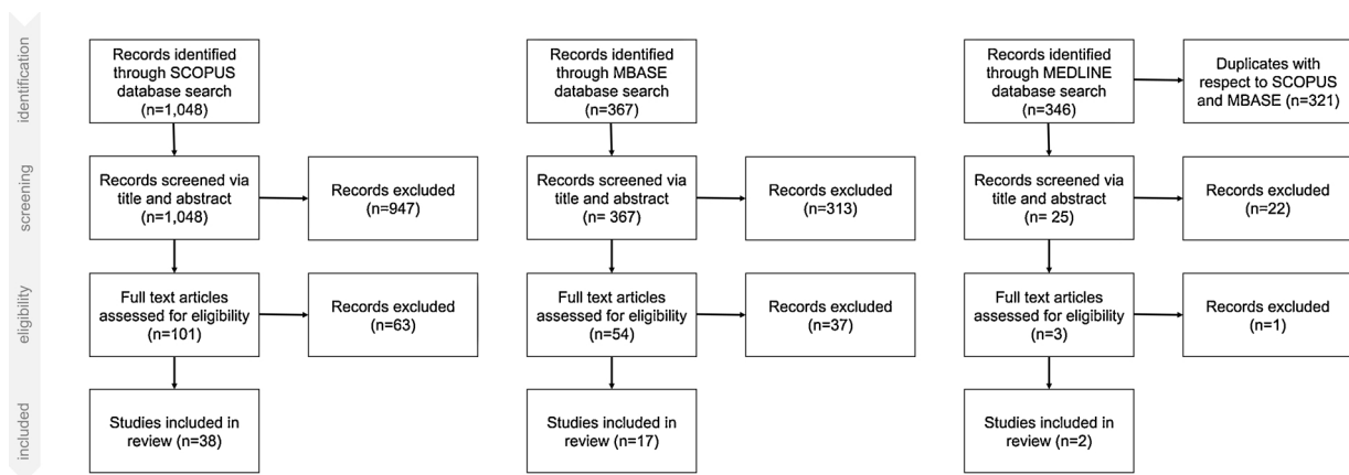
Fig. 1. Search strategy.
