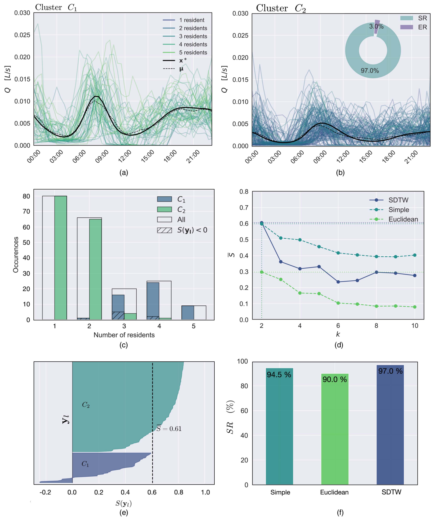
Fig. 5. Clustering results for SIMDEUM multiperson households obtained with SDTW clustering. SDTW: (a) family household cluster; (b) one- and two-person home cluster, all shown with barycenters x^* , cluster means \mu , and number of residents; (c) histograms for the resident distribution within the clusters; (d) cluster analysis plots; (e) silhouette plots for k = 2 for SDTW clustering; and (f) comparison of clustering performance with respect to SRs.
