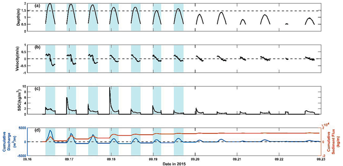
Fig. 3. Time series of (a) water depth (The dashed line represents the creek depth), (b) velocity (flood velocity is positive), (c) Suspended sediment concentration, and (d) cumulative discharge and sediment flux (into the creek is positive) in the main creek in September 2015. The overbank tides were highlighted in blue.
