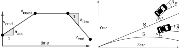
Fig. 4: Velocity profile
