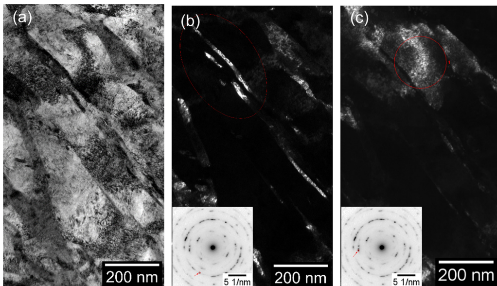
Fig. 8. TEM images taken from the necking area close to the fracture surface of the sample tested at a strain rate of 511 \text{ s}^{-1} . (a) Bright field (BF) image, (b) dark field (DF) image of interlath austenite, (c) DF image of martensite. Selected diffraction spots are marked with red color in the inserted diffraction patterns in (b) and (c), respectively.
