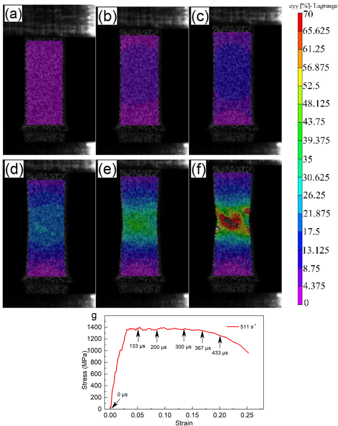
Fig. 5. Axial strain distribution obtained by DIC during a SHTB test at different times: (a) 0 \mu\text{s} , (b) 133 \mu\text{s} , (c) 200 \mu\text{s} , (d) 300 \mu\text{s} , (e) 367 \mu\text{s} , (f) 433 \mu\text{s} . (g) The corresponding engineering stress-strain curve for Fig. 5a to f. Arrows indicate times. The sample was tested at strain rate of 511 \text{s}^{-1} . (For interpretation of the references to color in this figure legend, the reader is referred to the Web version of this article.)
