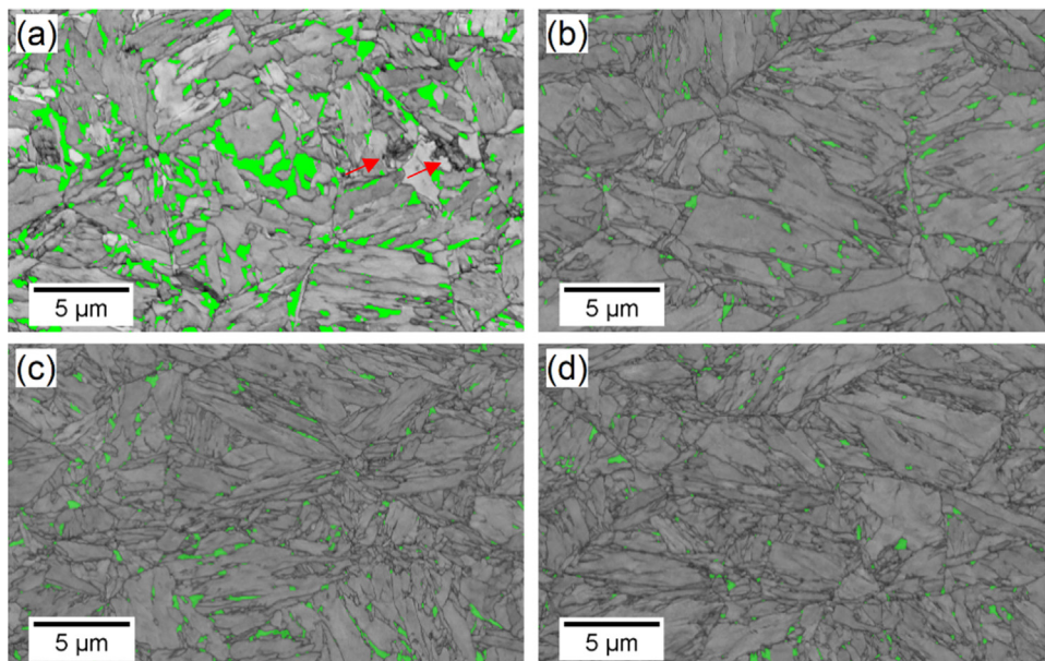
Fig. 7. Typical band contrast maps (combined with RA phase maps) for the studied Q&P steel at different true plastic strain: (a) 0, (b) 11.48%, (c) 16.66% and (d) 29.92%. The specimen was tested at strain rate of 511 \text{ s}^{-1} . Red arrows in Fig. 7(a) refers to untempered martensite. (For interpretation of the references to color in this figure legend, the reader is referred to the Web version of this article.).
