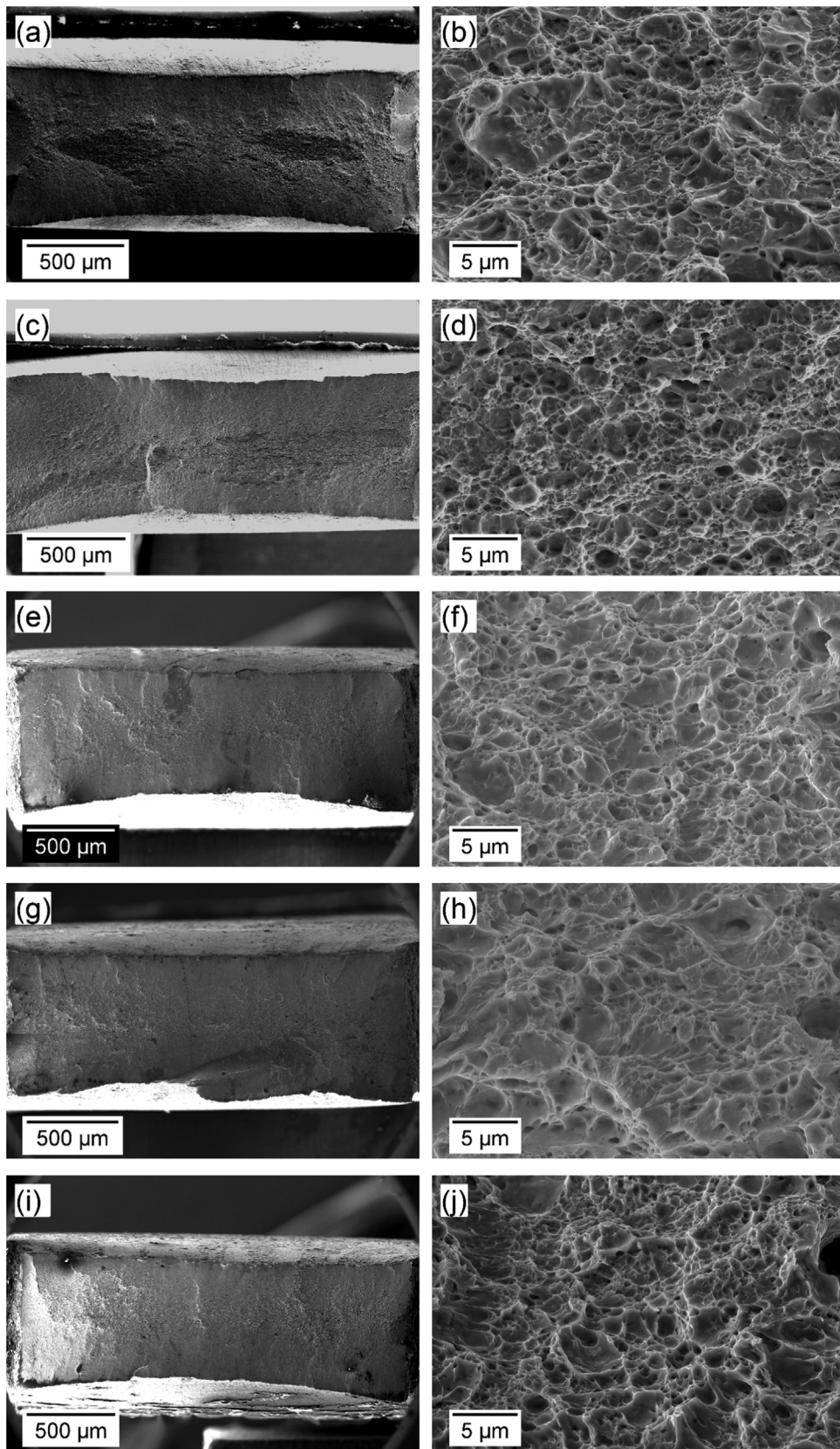
Fig. 10. Typical SEM images of fracture surfaces of the studied Q&P steel tested at strain rate of: (a, b) 1 \times 10^{-4} \text{ s}^{-1} , (c, d) 1 \times 10^{-2} \text{ s}^{-1} , (e, f) 511 \text{ s}^{-1} , (g, h) 742 \text{ s}^{-1} and (i, j) 962 \text{ s}^{-1} .
