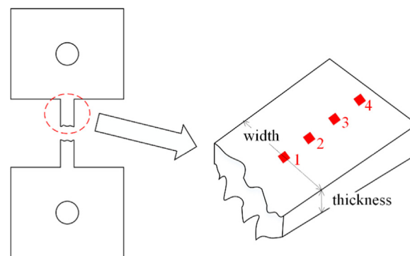
Fig. 3. Schematic presentation of the areas (marked by red squares) scanned by EBSD and the measurement of width and thickness after SHTB testing. The spacing between different areas was about 900\text{ }\mu\text{m} , and the first area was about 1 mm away from the fracture surface.
