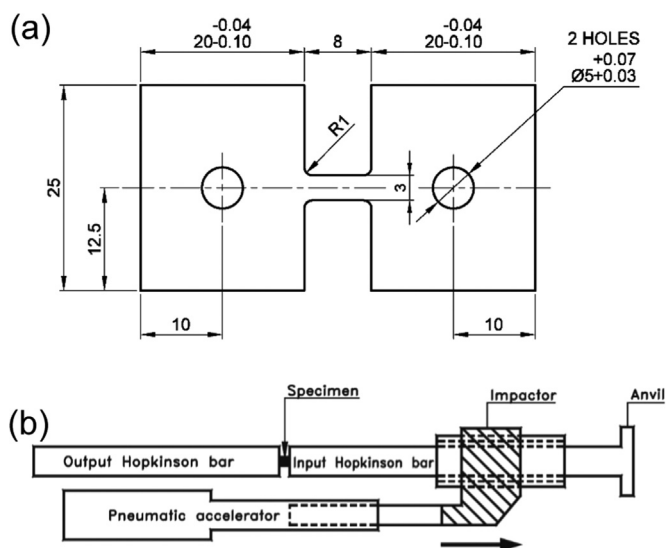
Fig. 2. (a) The geometry of specimens for static and dynamic tensile test; (b) Schematic presentation of the SHTB system.
