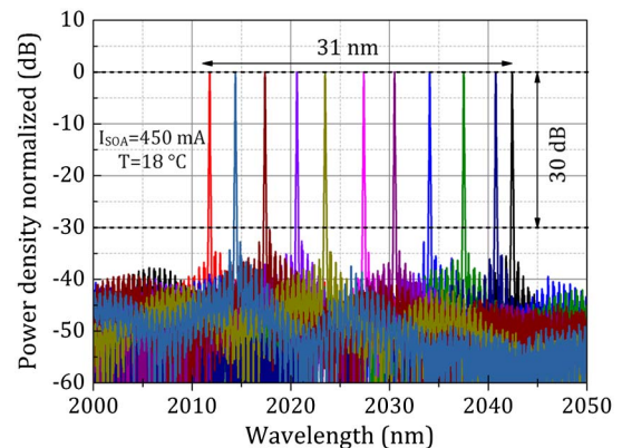
Fig. 6. Optical spectra recorded using an optical spectrum analyzer for different sets of reverse bias voltages applied to the ERM sections while both the injection current into the SOA section and the temperature were kept constant at I_{\text{SOA}} = 450 mA and T_{\text{HS}} = 18^\circ\text{C} , respectively. At such tuning conditions the laser covers a record tuning range of 31 nm.
