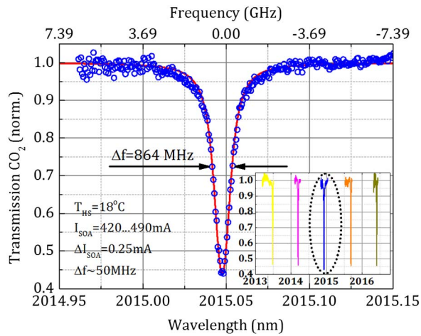
Fig. 7. Absorption line of CO 2 measured (blue circles) with the AMZI integrated tunable laser source and overlapped with the absorption profile simulated (solid red line) with the HITRAN software using parameters of the reference gas cell used for the experiment. The inset presents the measured absorption spectra of four more CO 2 transitions.
