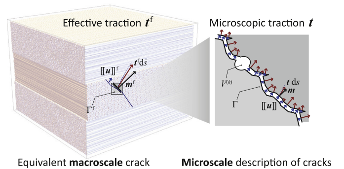
Fig. 3. Illustration of a sub-ply volume element with a microscopic crack (right) and equivalent macroscale crack (left) with effective normal vector \mathbf{m}^f , effective cohesive traction \mathbf{t}^f and effective crack opening \llbracket \mathbf{u} \rrbracket^f . Observe that here the notion of macroscale refers to a larger scale compared to the microscale but still within a single ply in a laminate.
