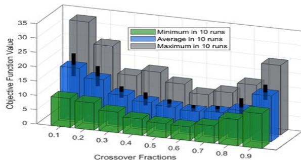
Fig. 5. 3-D Bar graph illustrating the objective function values averaged over 10 runs for 9 different Crossover Fraction values.
