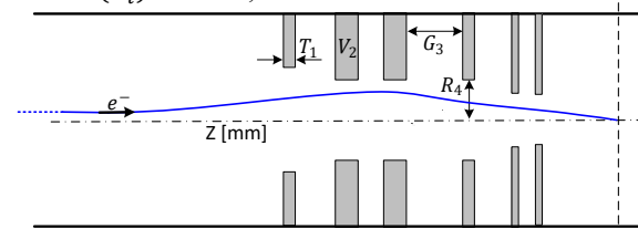
Fig. 1. A 2D illustration of a typical multi-electrode lens systems with 6 electrodes.
