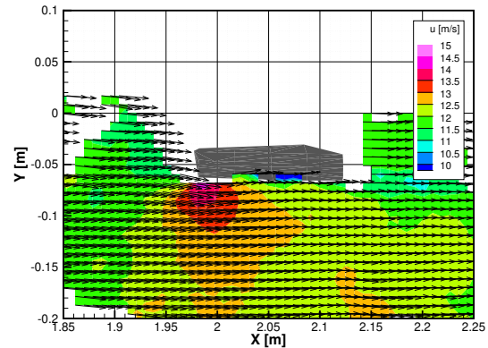
(d) 2D top view at t/T_{ref} = 1
