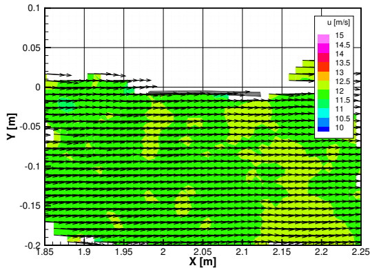
(c) 2D top view at t/T_{ref} = 0.75
