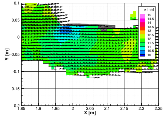
(b) 2D top view at t/T_{ref} = 0.5
