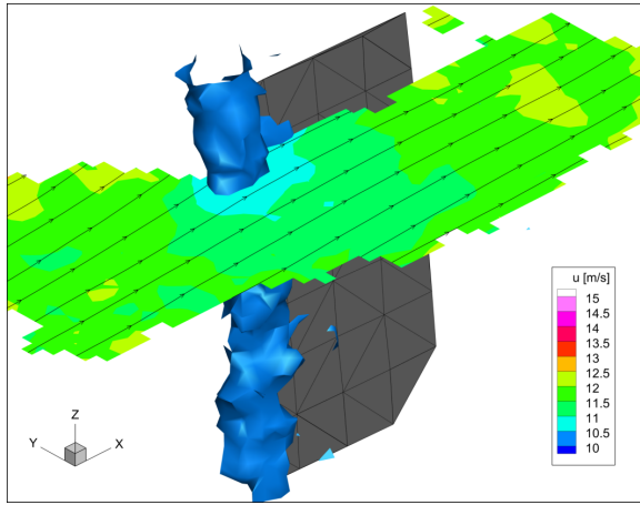
(a) 3D view at t/T_{ref} = 0.5 . Iso-surface of u = 10.5 m/s
