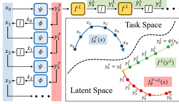
Figure 5.3.: Structure of CONDOR. We show an example of discrete-time trajectories generated with f_\theta^T , f^L and f_\theta^{T \rightarrow L} before training the DNN. Starting from an initial point x_0 , a trajectory is generated in \mathcal{T} using f_\theta^T (blue) and two trajectories are generated in \mathcal{L} . One of them follows f_\theta^{T \rightarrow L} (red), and the other follows f^L (green).
