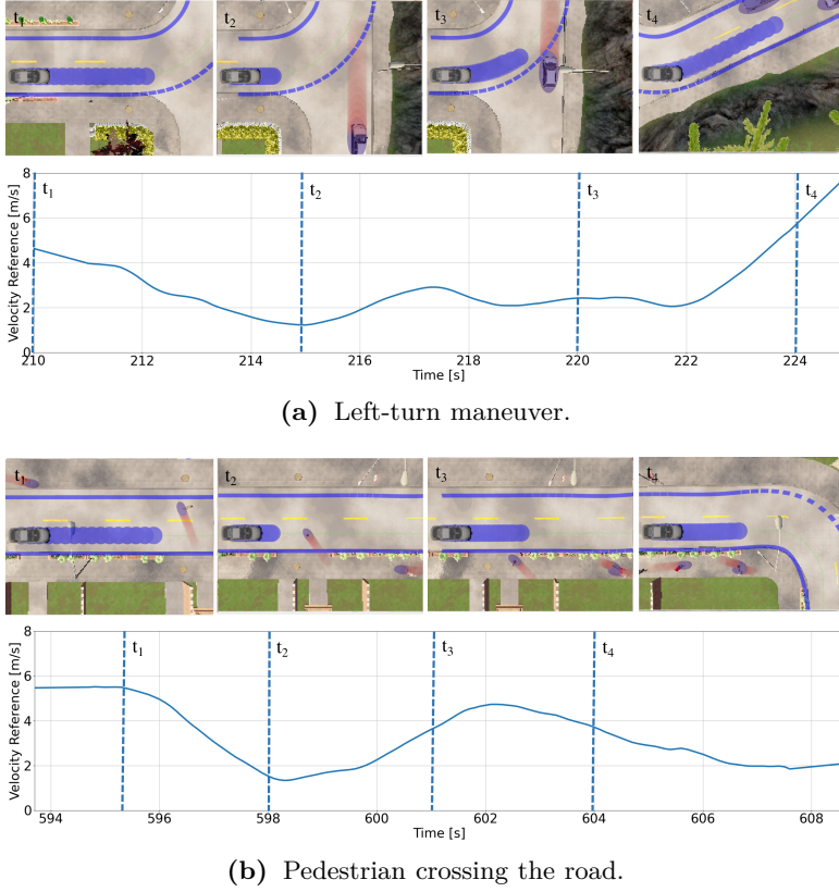
Figure 4.5.: The blue circles depict the MPCC’s velocity reference provided by the VG and the blue lines the road constraints. The red circles depict the predicted constant velocity trajectory for the other vehicles or pedestrians.
