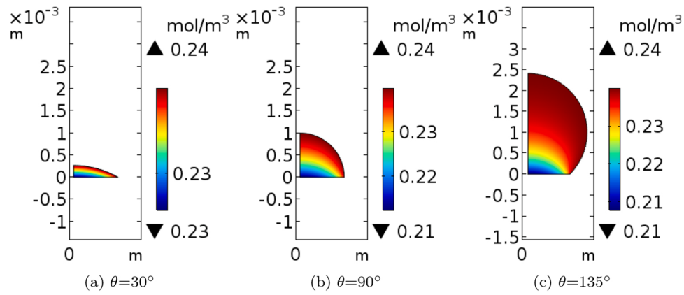
Fig. 8. O_2 concentration profiles for three different contact angles ( \theta = 30^\circ , 90^\circ and 135^\circ ) for a wetted radius of 1 mm. The difference in contact angle causes different aeration and thus different oxygen accessibility.
