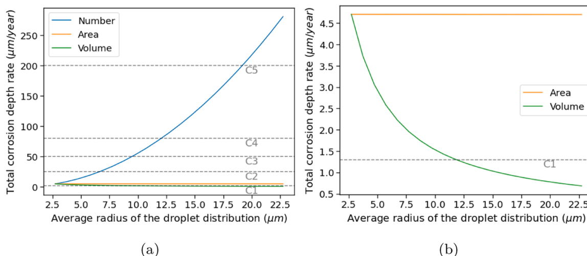
Fig. 20. Thickness loss rate on iron as a function of the average droplet distribution radius under different conditions over the surface.
