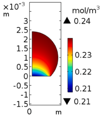
Fig. 2. Axisymmetric geometry of a droplet used in this work. The colorscale indicates the steady-state oxygen concentration ( \text{mol/m}^3 ) resulting on iron in a droplet with a radius of 1 mm and a contact angle of 135^\circ .
