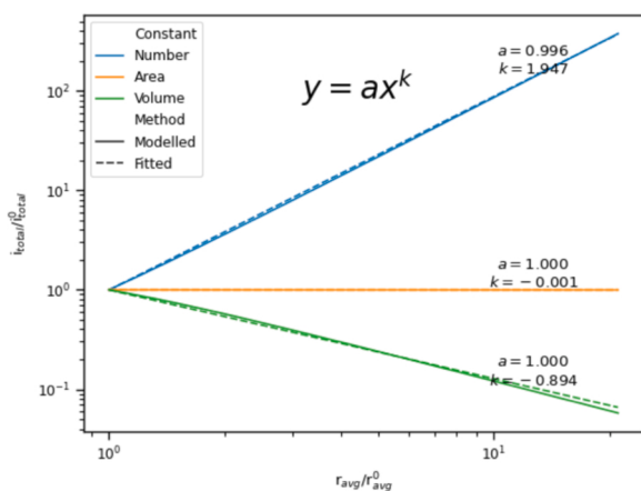
Fig. 17. Comparison of the corrosion current density change as function of the average droplet radius.
