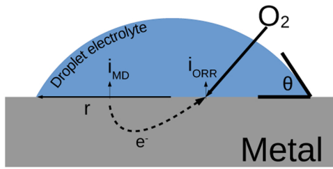
Fig. 1. Illustration of the oxygen reduction and metal dissolution current densities in a droplet with r the droplet radius, \theta the contact angle, i_{MD} and i_{ORR} the metal dissolution and oxygen reduction current densities, respectively.
