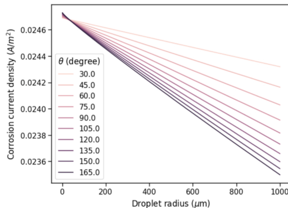
Fig. 11. Averaged corrosion current densities for iron as function of the contact angle and droplet radius.
