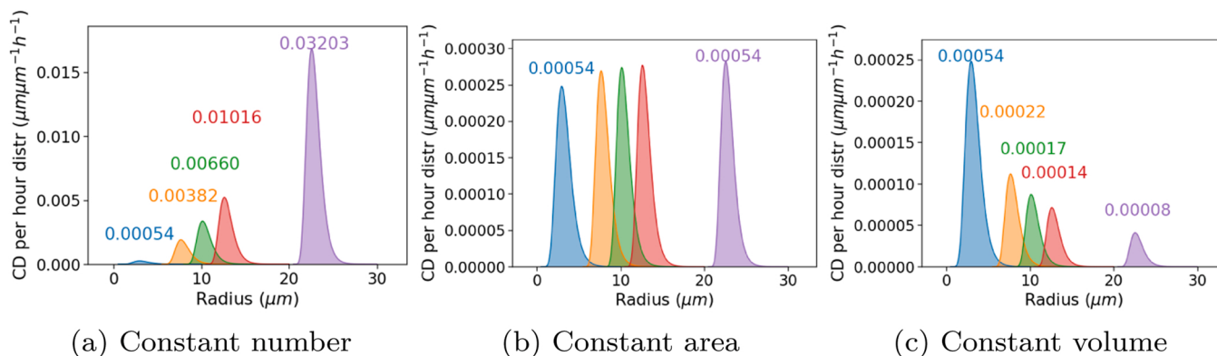
Fig. 19. Corrosion rate for different distributions on iron. The integrated (total) corrosion rate is indicated above in \mu\text{m}/\text{h} .
