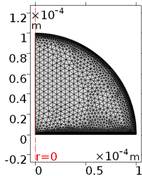
Fig. 3. The mesh for a single droplet simulation.
