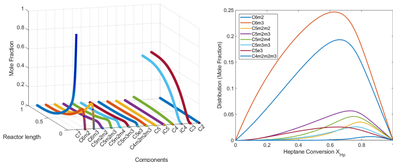
Fig. 8. Left: Normalized molar concentration (mol per mol of C_7 feed) of different components plotted as a function of the reactor length with n -heptane feedstock. Right: Normalized molar concentration (mol per mol of C_7 feed) of various n -heptane isomers as a function of heptane conversion for simulations conducted at 594 K.
