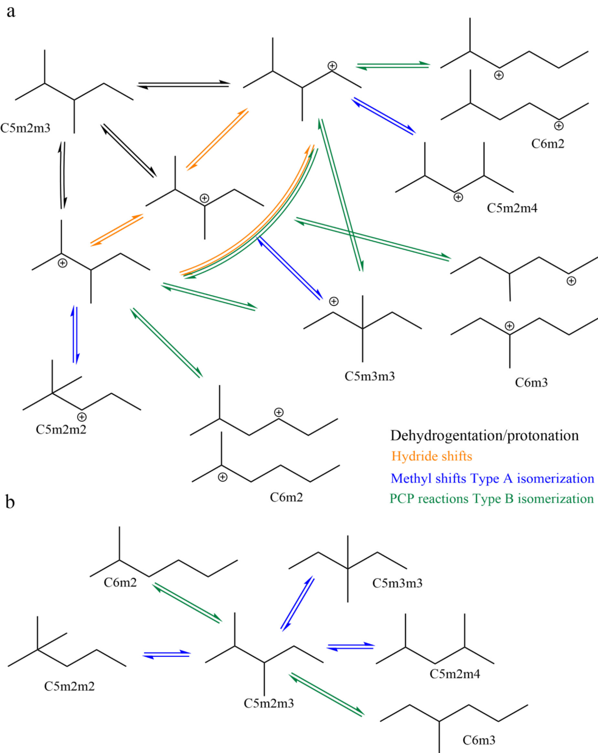
Fig. 3. (a) Illustration of all possible isomerization pathways for 2,3-dimethyl-pentane with dehydrogenation and protonation followed by backbone isomerization of type A (methyl or ethyl shift, blue arrows) or type B (branching isomerization, green arrows). (b) Reaction pathways used to model isomerization reactions associated with 2,3-dimethyl-pentane in our reaction network. (For interpretation of the references to colour in this figure legend, the reader is referred to the web version of this article.)
