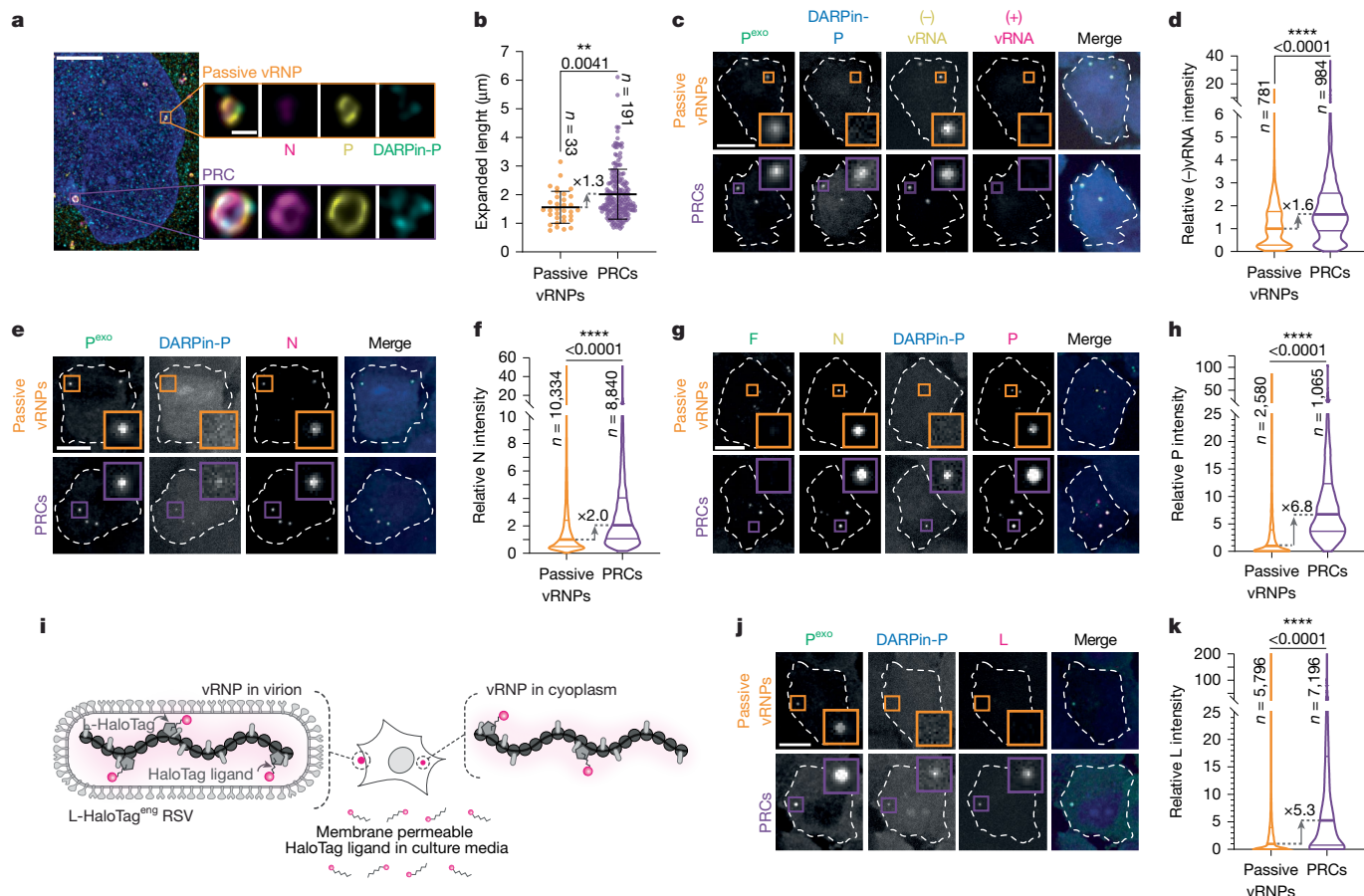
Fig. 5 | PRCs have higher quantities of associated viral proteins. Incoming passive vRNPs and PRCs were assessed at 4 h following viral inoculum addition. The translation inhibitor emetine was added to cells together with virus addition to prevent progression of infection. a, b , Super-resolution imaging of RSV vRNPs by ExM (approximately \times 4.5 ). Representative images ( a ) and quantification ( b ) highlight size differences between passive vRNPs and PRCs. c, d , Genome ((-)vRNA) and antigenome ((+)vRNA) presence in vRNPs was evaluated. Representative images of smFISH staining carried out on the P exo -fluoro/DARPin-P-fluoro cell line ( c ) and quantification of the (-)vRNA intensity for passive vRNPs and PRCs ( d ) are shown. e–k , RSV vRNP-constituent protein levels were assessed in passive vRNPs and PRCs. Representative images ( e ) and quantification ( f ) of N levels. Representative images ( g ) and quantification ( h )
