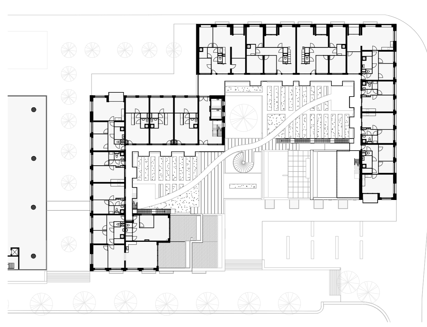
Level 5
