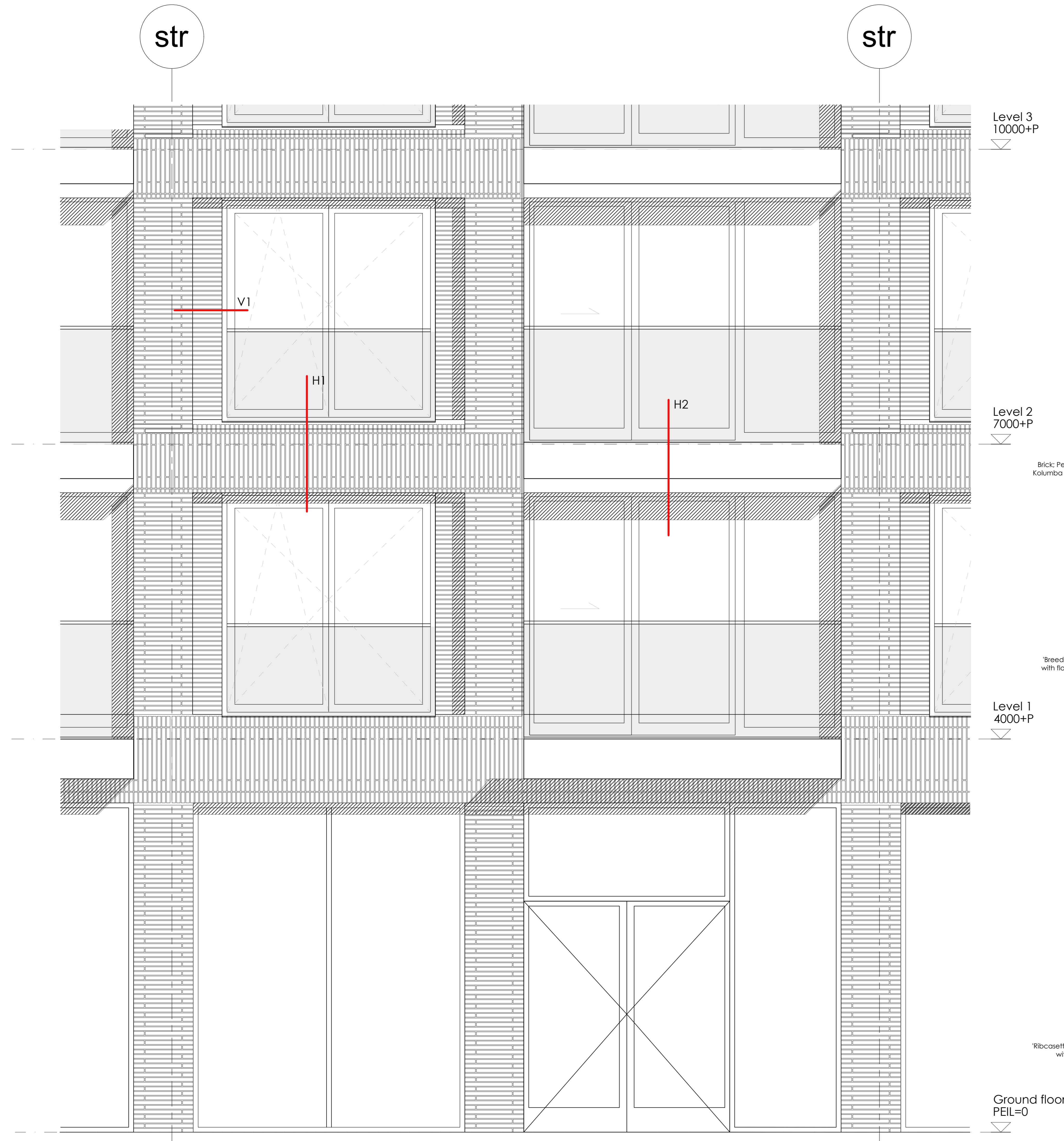
Facade fragment 1 : 20
