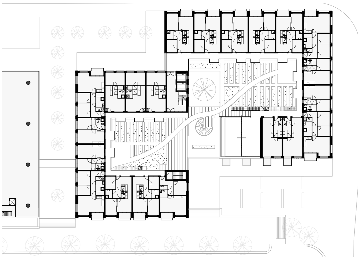
Level 3
