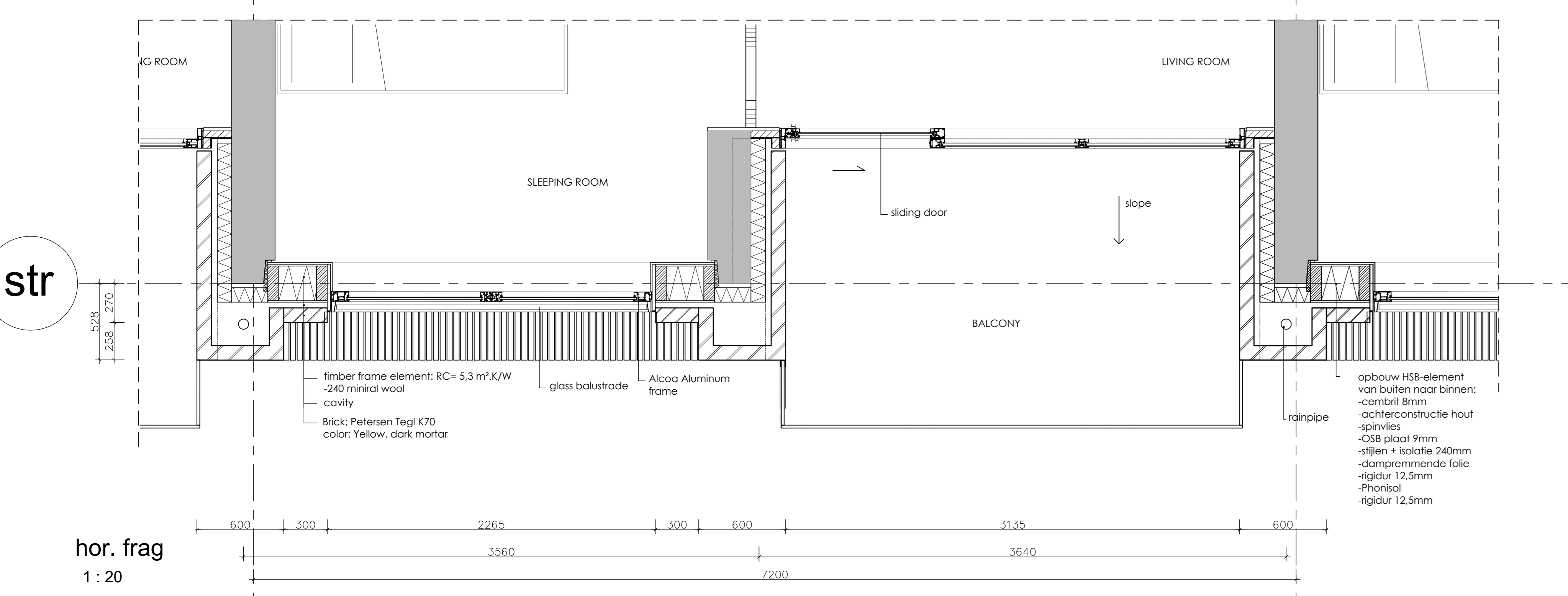
Facade fragment 1 : 20
