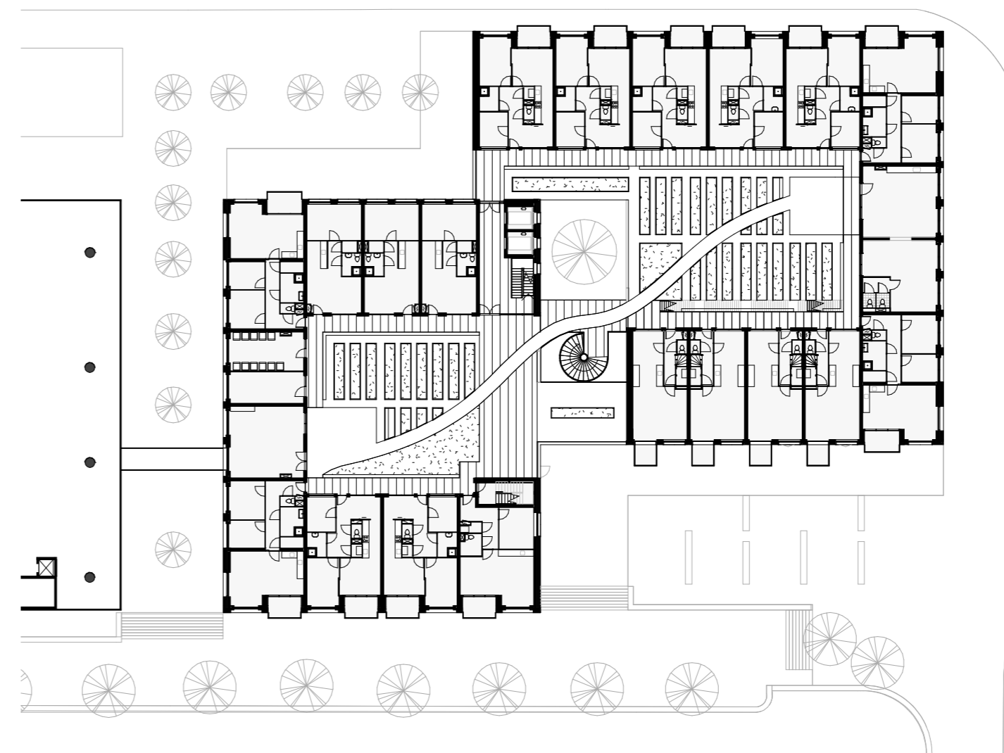
Level 1
