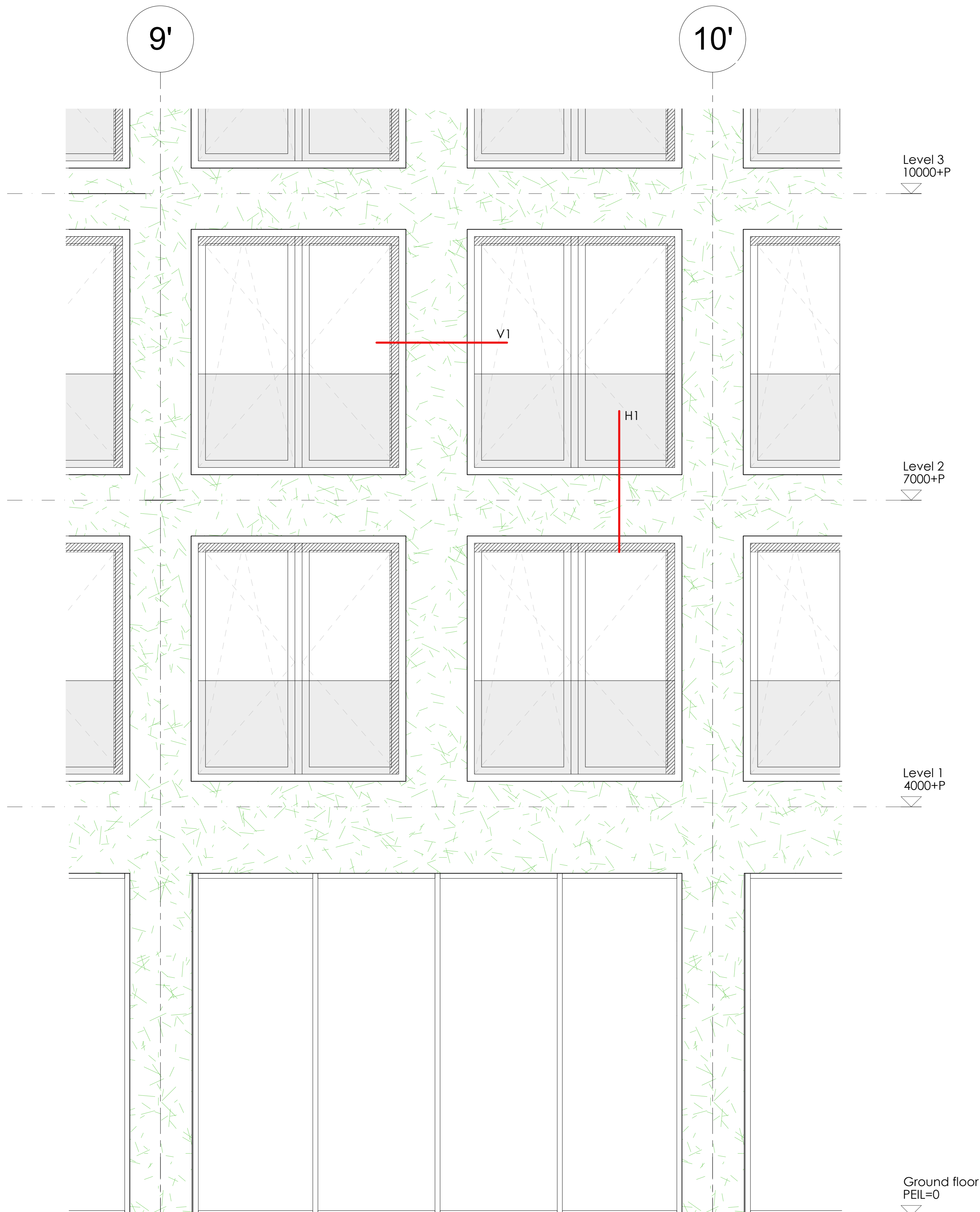
Facade fragment 1 : 20
