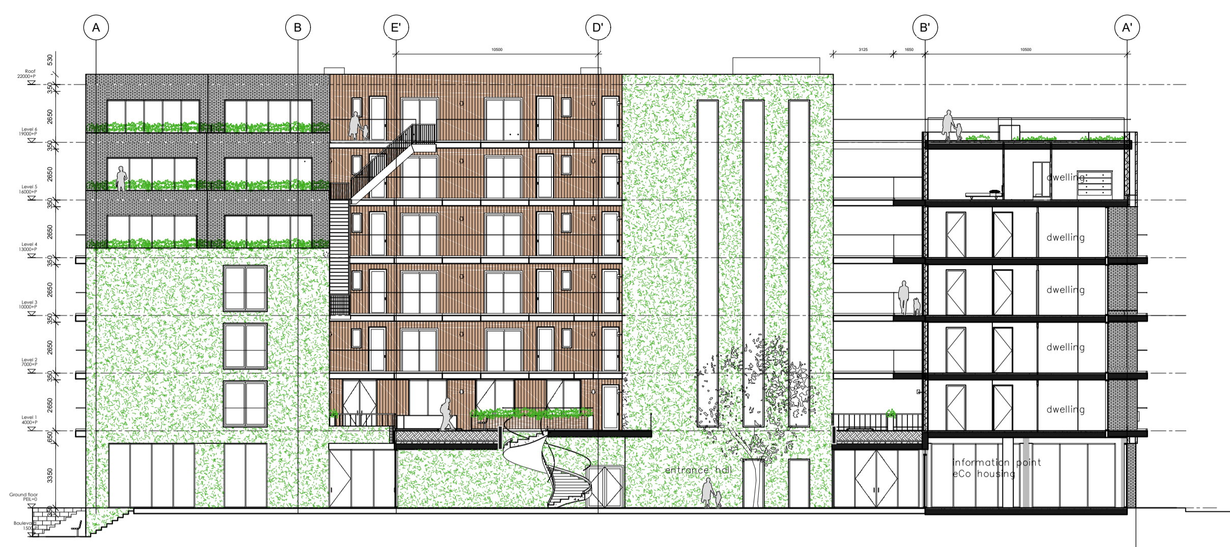
Section FF
