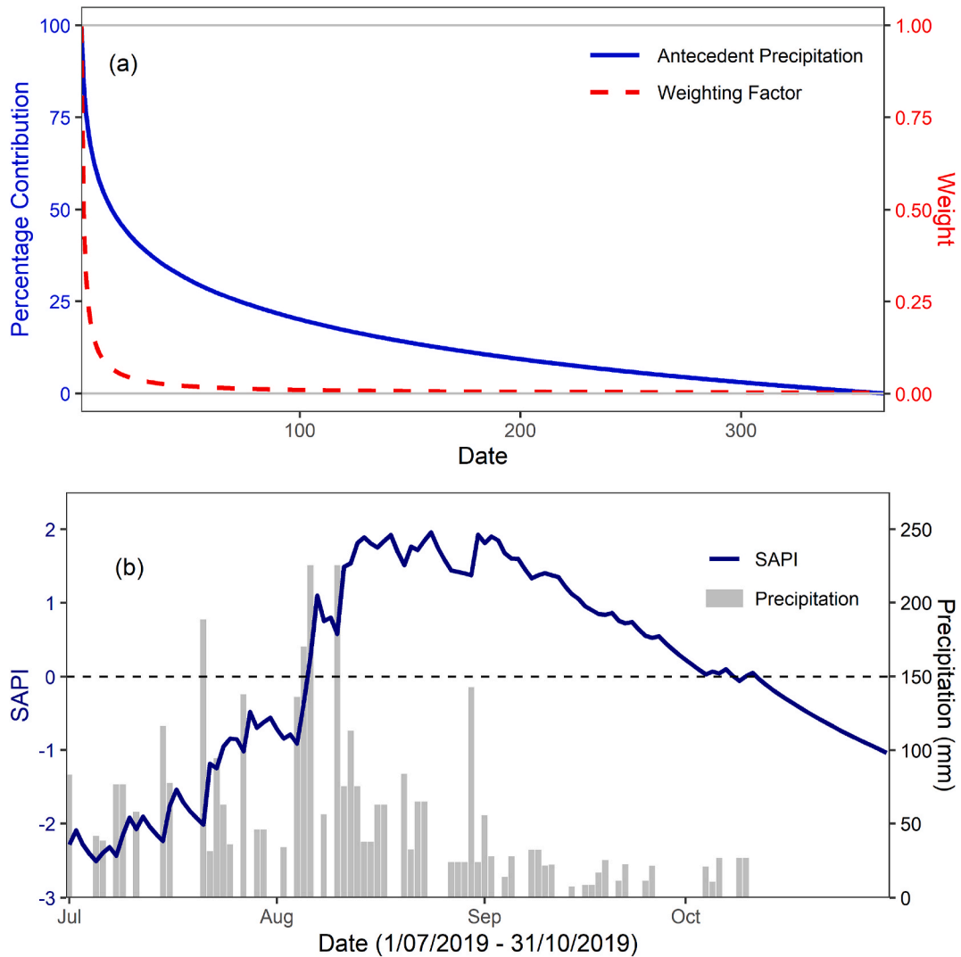
Fig. 2. (a) The time-dependent reduction function showing ratio of weighted contribution of raw precipitation ( P ) into effective precipitation ( P_e ) over annual cycle ( N = 365 days). (b) An example of duration, volume, and peak of the Standardized Antecedent Precipitation Index (SAPI) time series extracted at Bilin town ( 17.225^\circ N, 97.225^\circ E) in Mon state, Myanmar. A flood event is defined as when SAPI > 0 .
