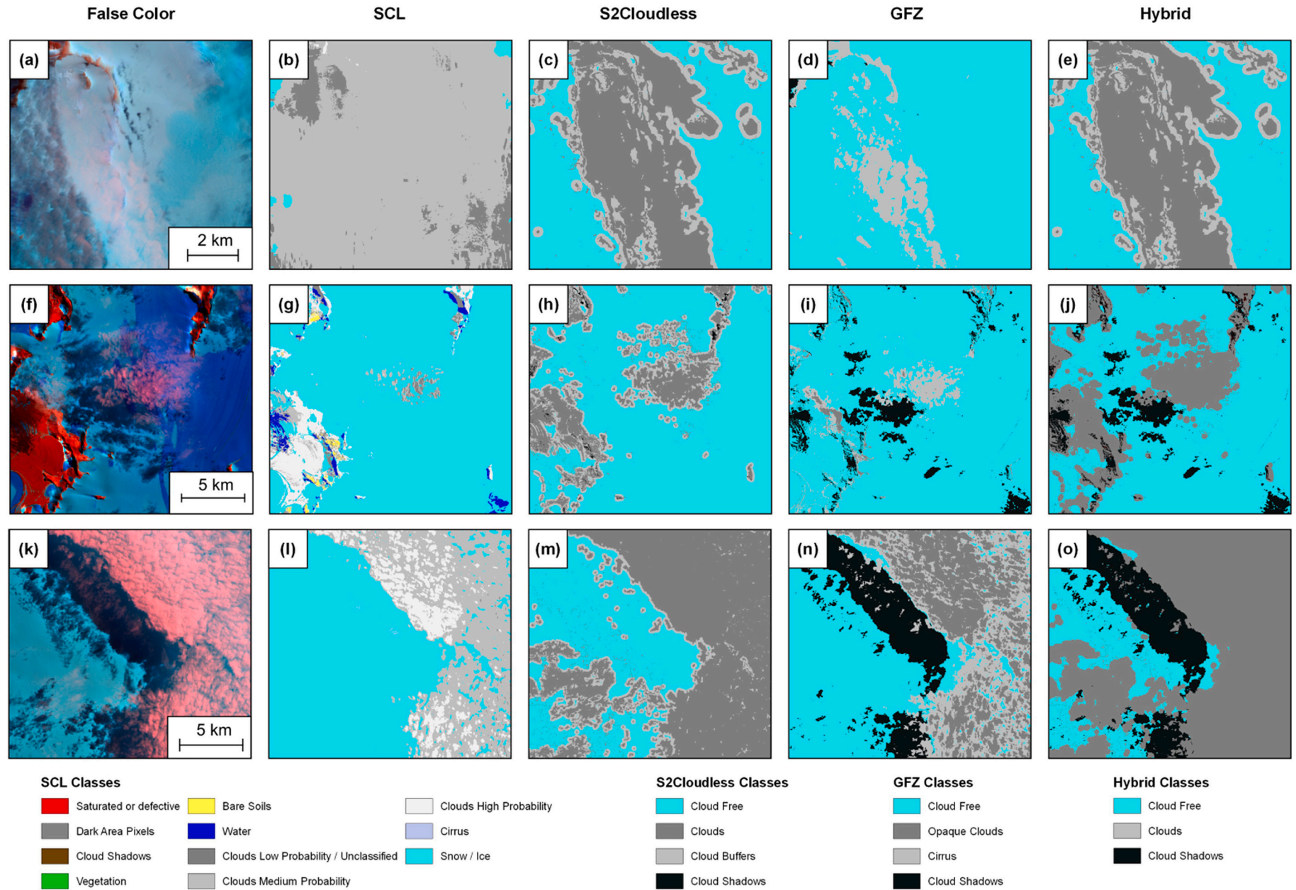
Fig. A.14. Cloud masks for Sentinel-2 imagery based on the scene classification map (SCL), s2cloudless, GFZ method, and hybrid method, under different cloudiness: hazy (a-e), partially cloudy/hazy (f-j), heavily cloudy (k-o).
