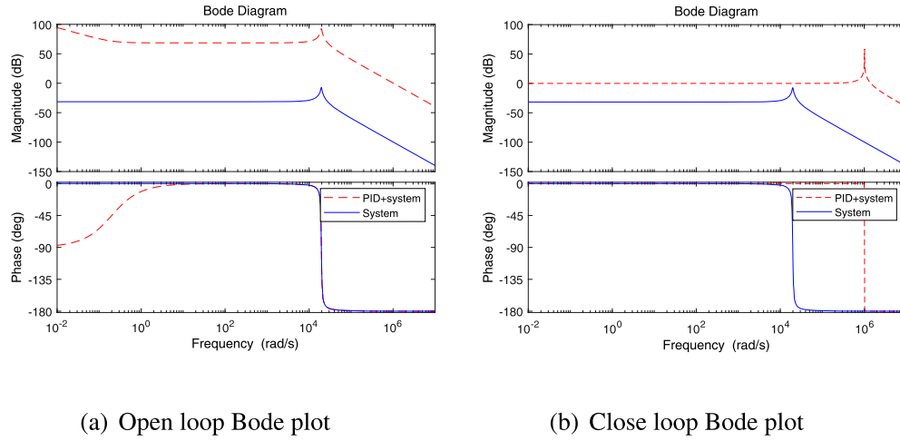
Fig. 14. Bode plots of the linearized system at the working condition of \dot{m} = 0 .
