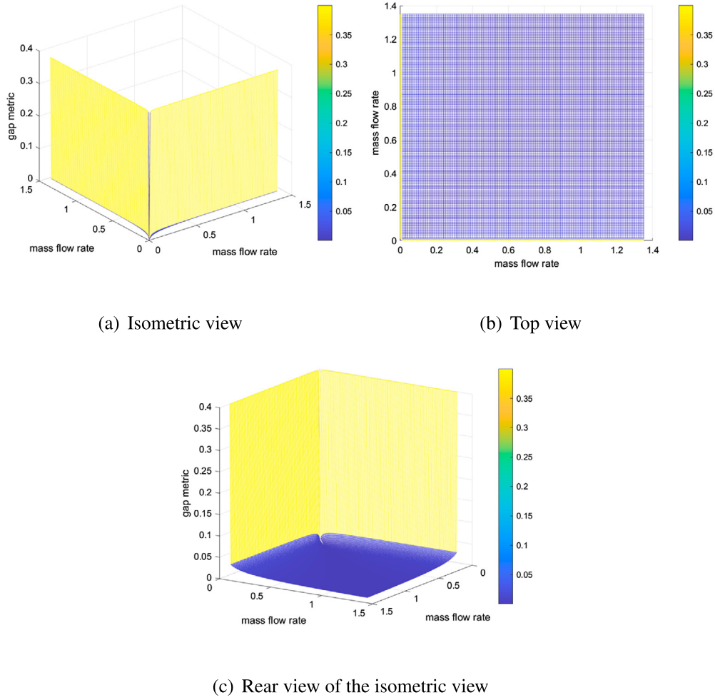
Fig. 1. Gap metric surface of the system ( \dot{m} \in [0, 1.35] ). (For interpretation of the colors in the figure(s), the reader is referred to the web version of this article.)
