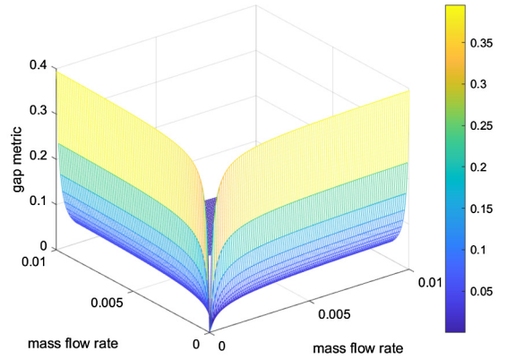
Fig. 3. Gap metric surface of the system ( \dot{m} \in [0, 0.01] ).
