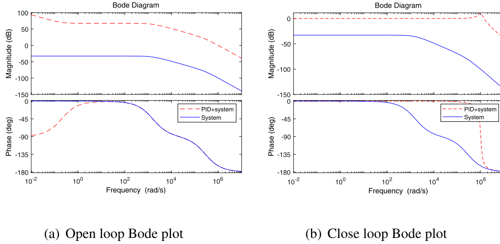
Fig. 13. Bode plots of the linearized system at the working condition of \dot{m} = 0.03 kg/s.
