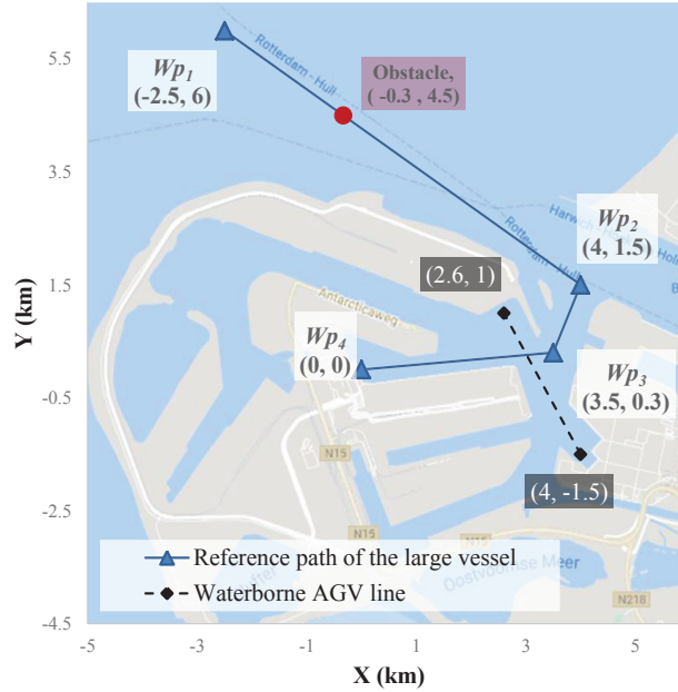
Figure 5.6: Reference paths in the simulation experiments.
