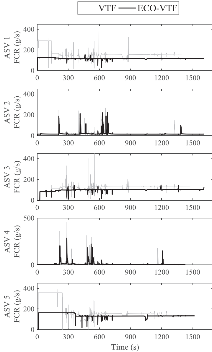
Figure 4.23: Fuel consumption rate of each ASV.
