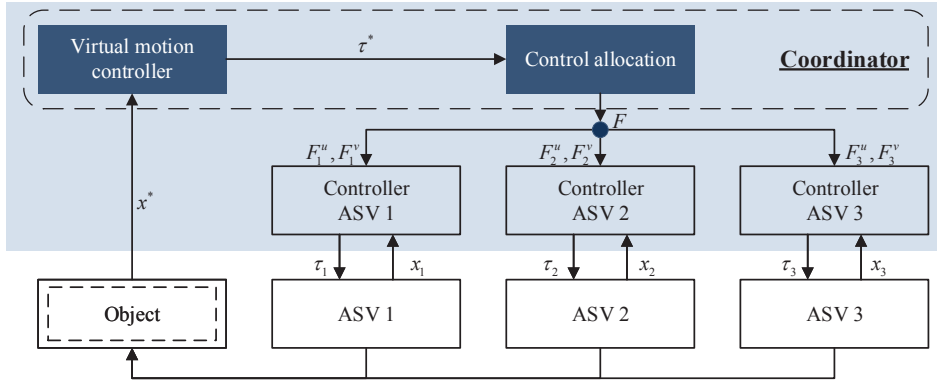
Figure 5.3: Multi-layer DMPC for cooperative object transport.
