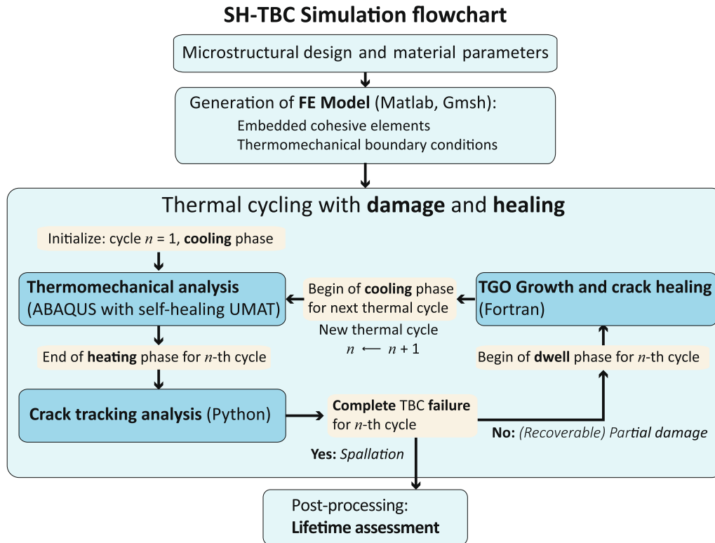
Fig. 3. Overall simulation procedure for self healing TBC system. The TGO growth and crack healing process occurs mostly during the dwell phase, whereas most of the damage occurs during the cooling phase.
