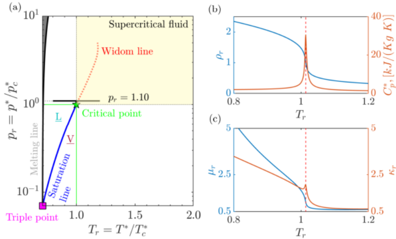
Figure 1: (a) Pressure-temperature ( p - T ) diagram of \text{CO}_2 along with the triple point (magenta), critical point (green), saturation line (blue), Widom line (red line) and supercritical fluid region ( \text{sCO}_2 ) in yellow. At a reduced pressure of p_r = 1.10 as a function of reduced temperature T_r : (b) reduced density \rho_r and dimensional specific heat C_p^* , (c) reduced viscosity \mu_r and reduced thermal conductivity \kappa_r . The Widom line (---) is at T_{pc}^* , or T_{r,pc} = 1.024 .
